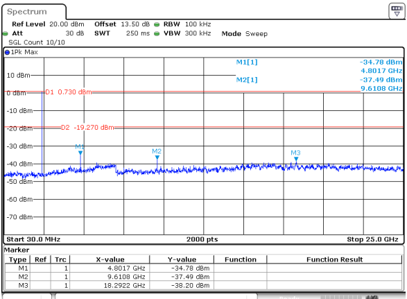
BLE_2M_Low_Channel
