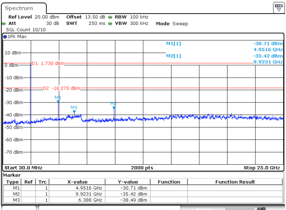
BLE_2M_High_Channel
