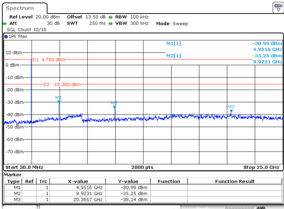
BLE_1M_High_Channel
