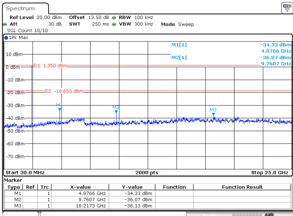
BLE_2M_Middle_Channel
