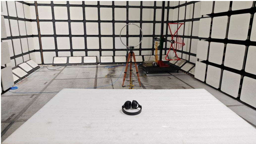
Radiated Emissions View (Below 30MHz)
