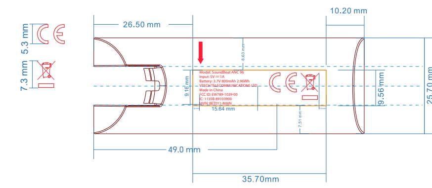
L side inner silkscreen
