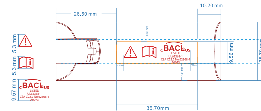
R side inner silkscreen
