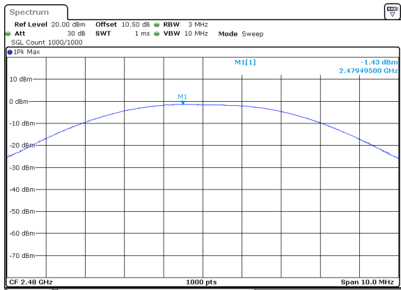
BLE_2M_High_Channel
