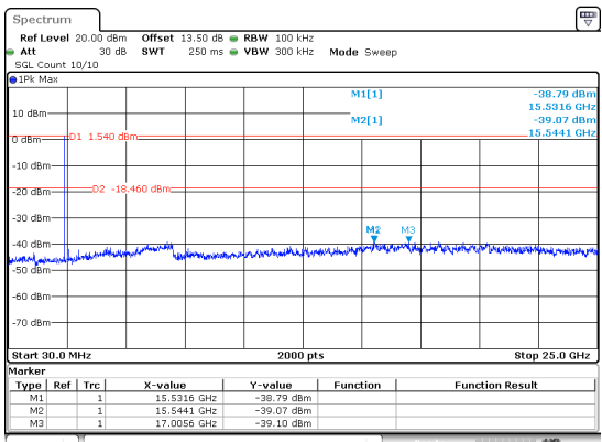
BLE_1M_Low_Channel
