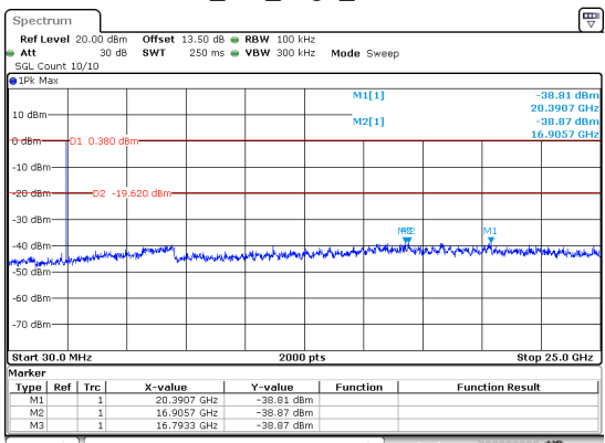
BLE_1M_High_Channel
