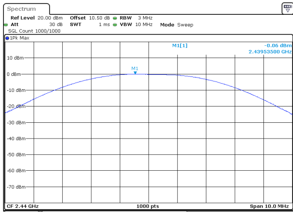
BLE_2M_Middle_Channel
