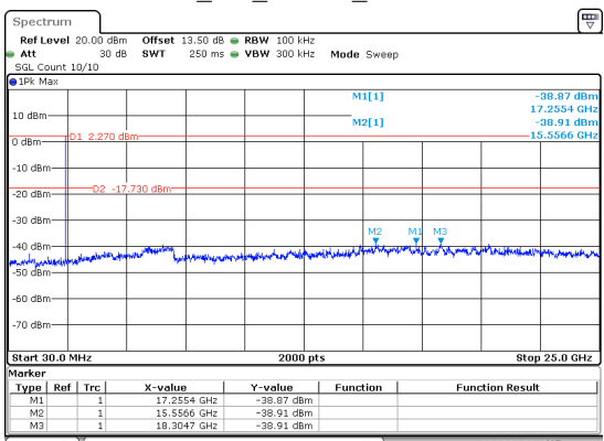
BLE_2M_Middle_Channel
