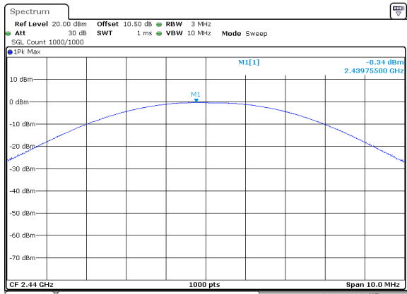
BLE_1M_Middle_Channel
