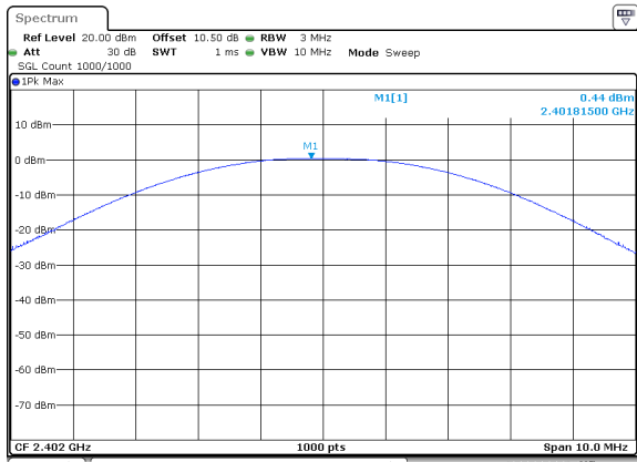
BLE_1M_Low_Channel
