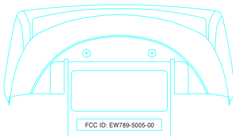
XX-9122 HANDSET BOTTOM VIEW (COMMON TO ALL COLOUR)
