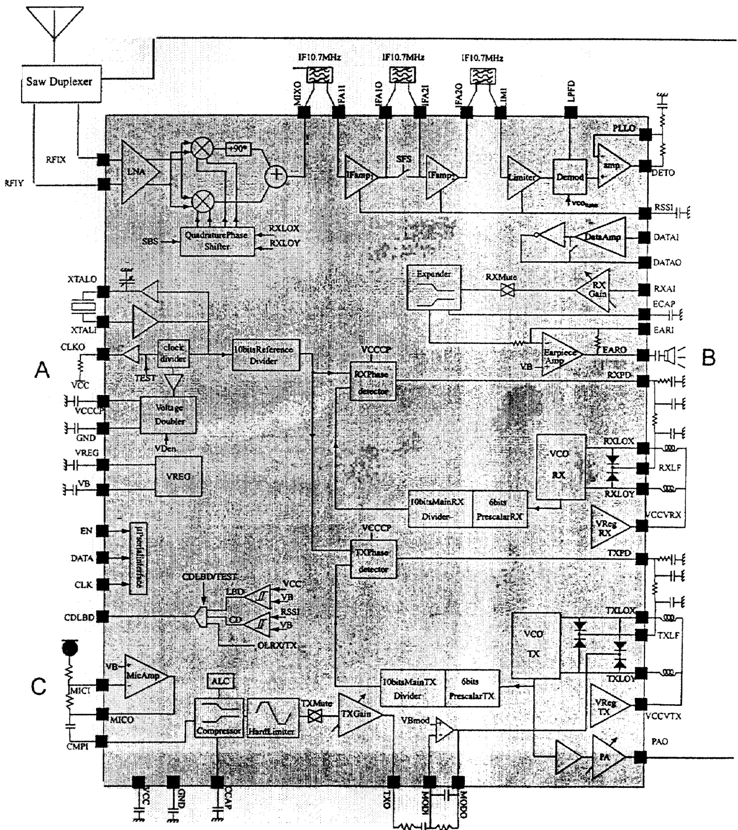
Figure 3. RF Module Block Diagram of Base and Handset.
