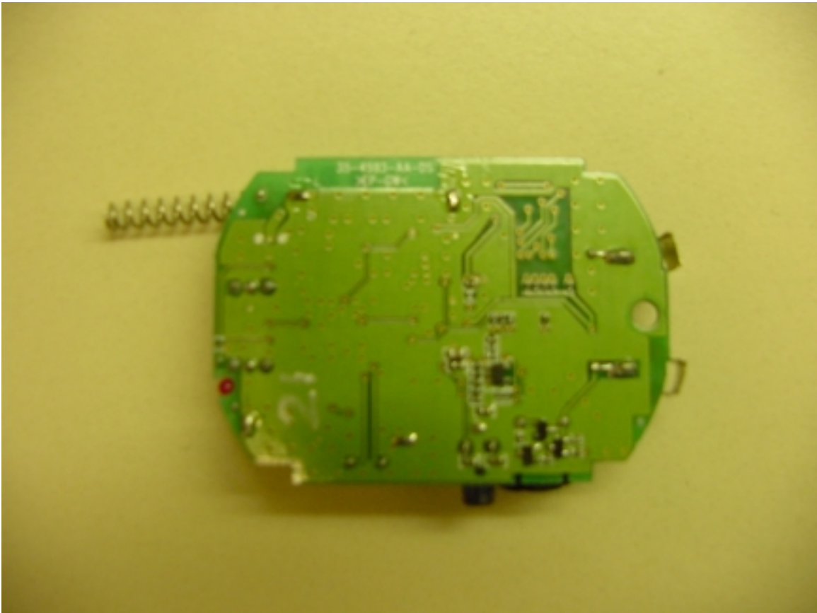
Back of Circuit Board for Handset
