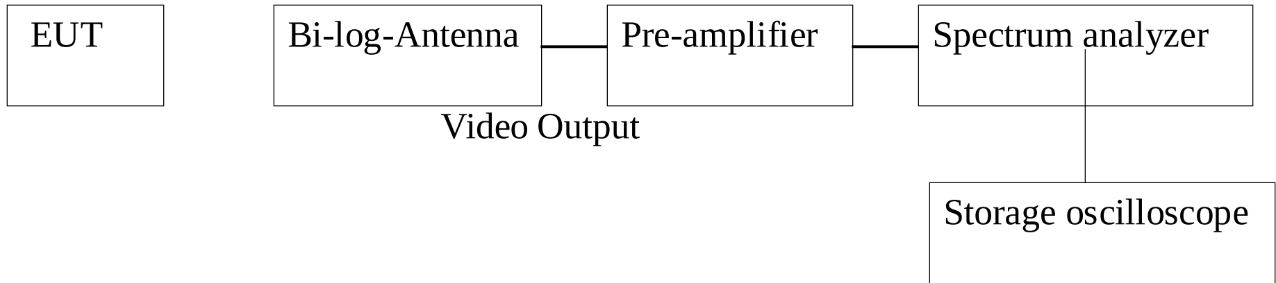
Block diagram for Duty Cycle calculation
