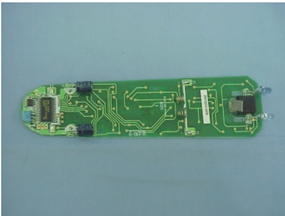
FIGURE 4 UHF/IR Remote Controller (M/N: EW7DVD15) BOARD 1 (COMPONENT SIDE)
