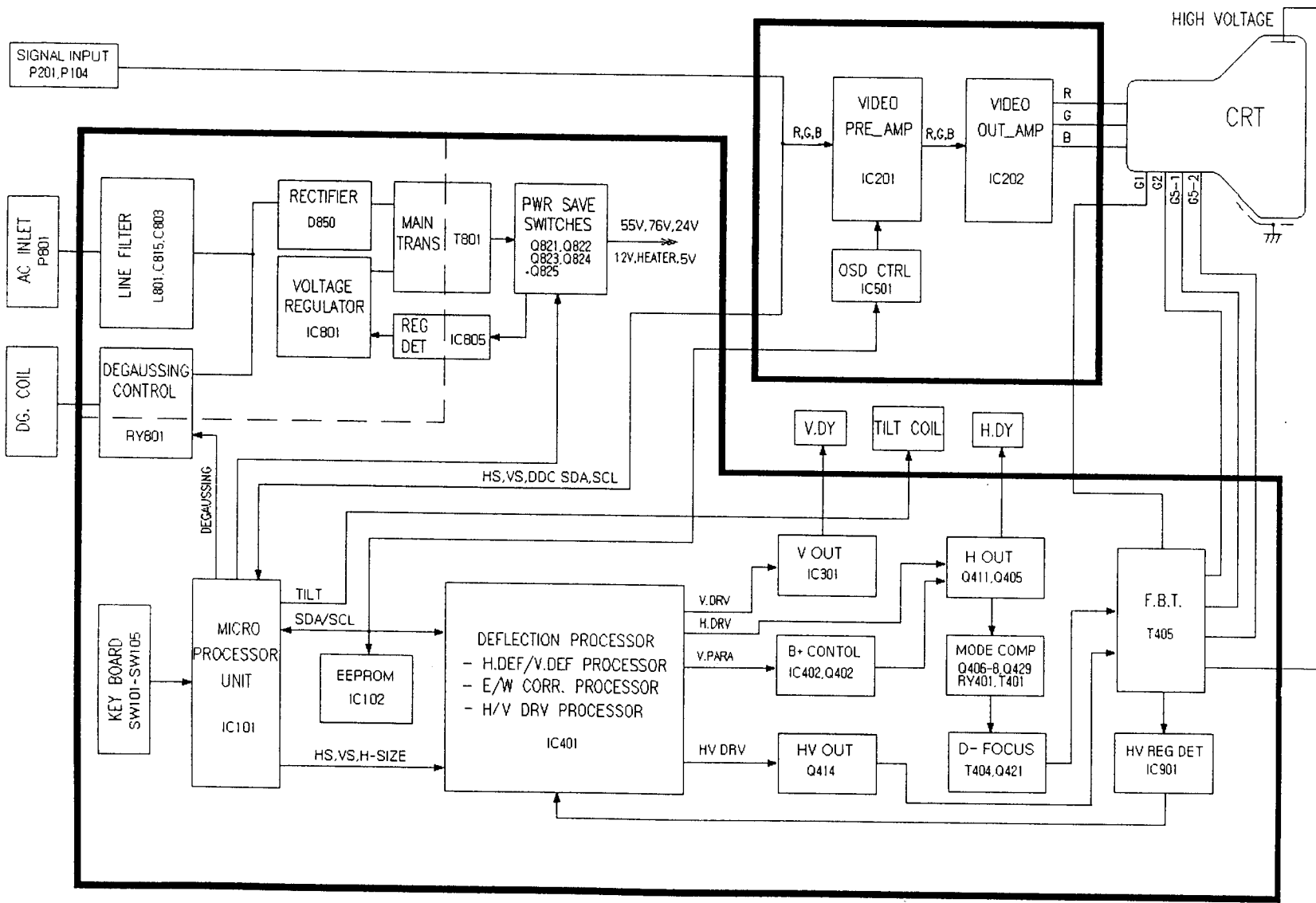
2. Block Diagram
