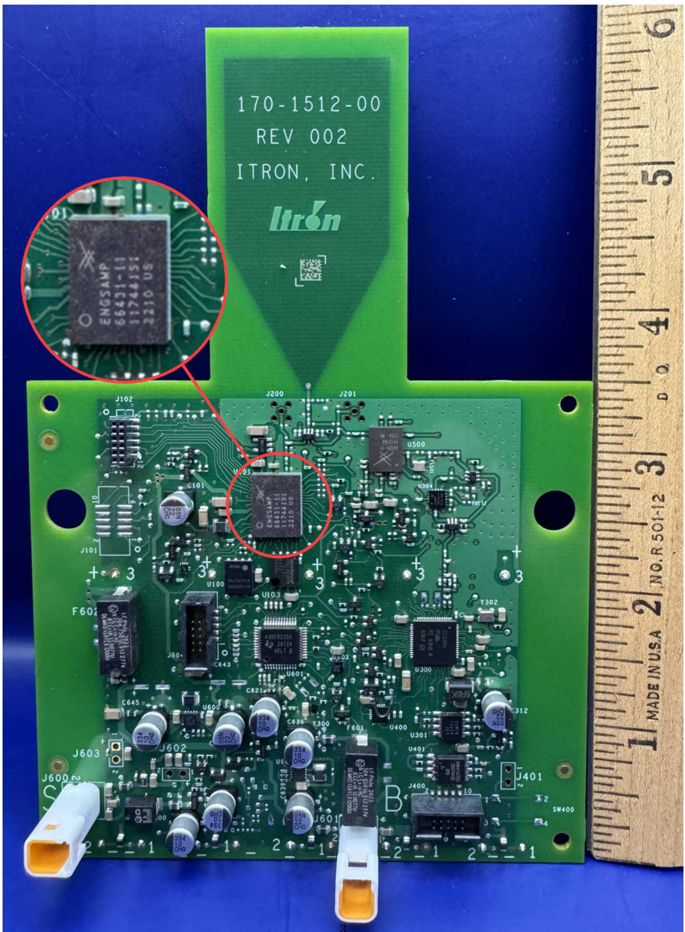
Figure 1.1: PCB Front
