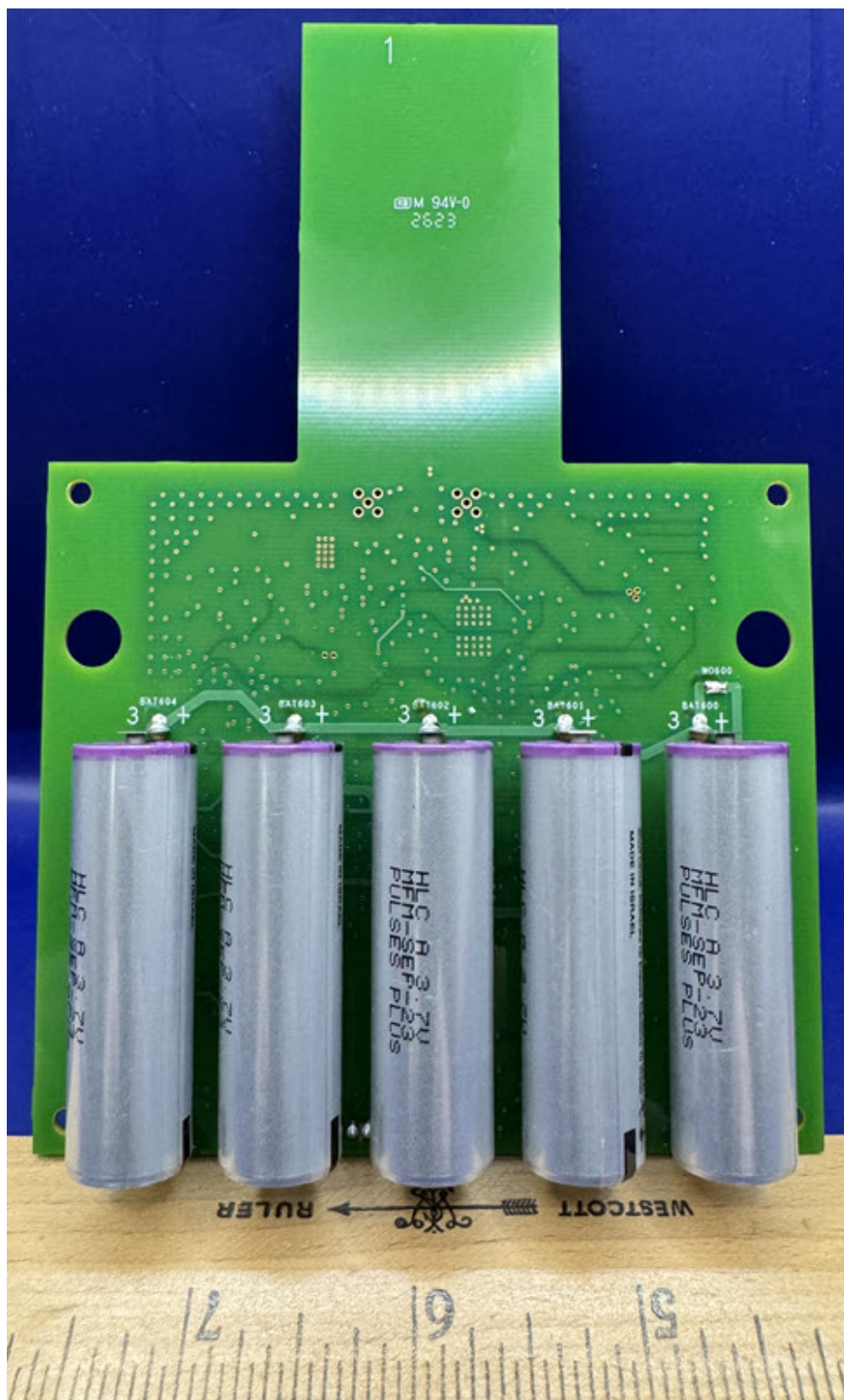
Figure 1.2: PCB Back
