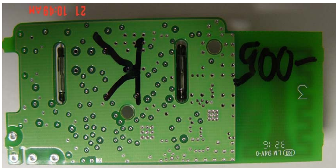
Bottom Side of PCB-5006-001 used in 100GDLAS and 100GDLCS
