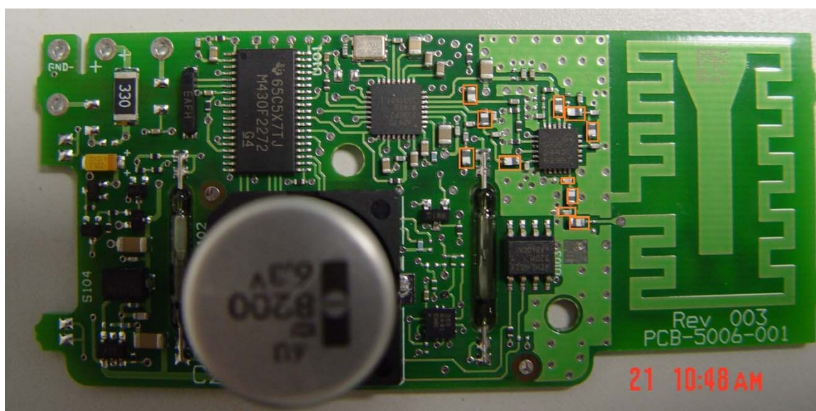
Parts Changed on PCB-5006-001 used in E100GDLAS and 100GDLCS;
