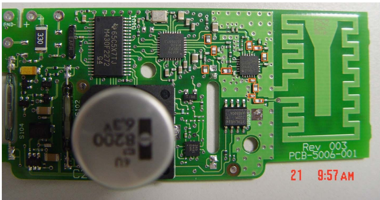
Parts Changed on PCB-5006-001 used in 100GDLBS
