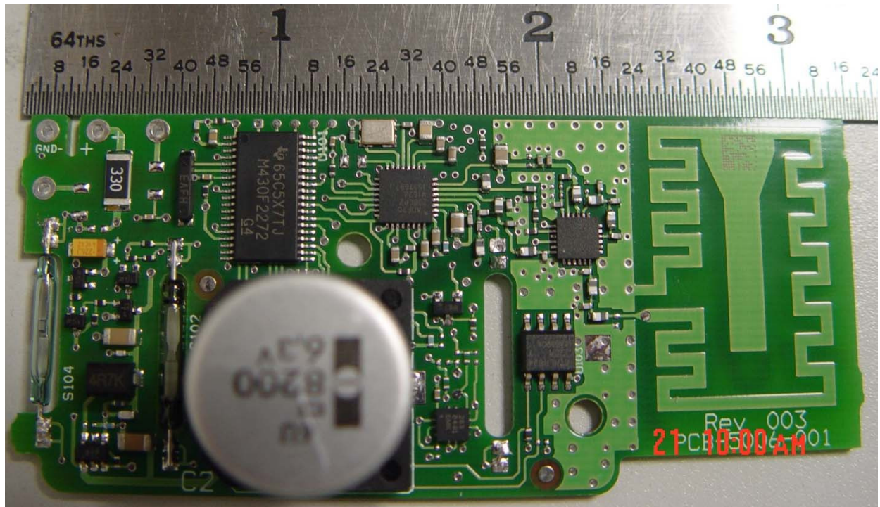
Top Side of PCB-5006-001 used in 100GDLBS
