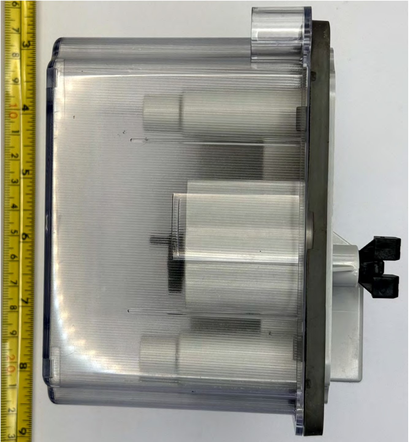
Figure 6.6: ERG-5600-009 External Bottom
