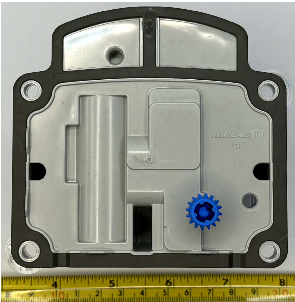
Figure 4.4: ERG-5600-003 External Back
