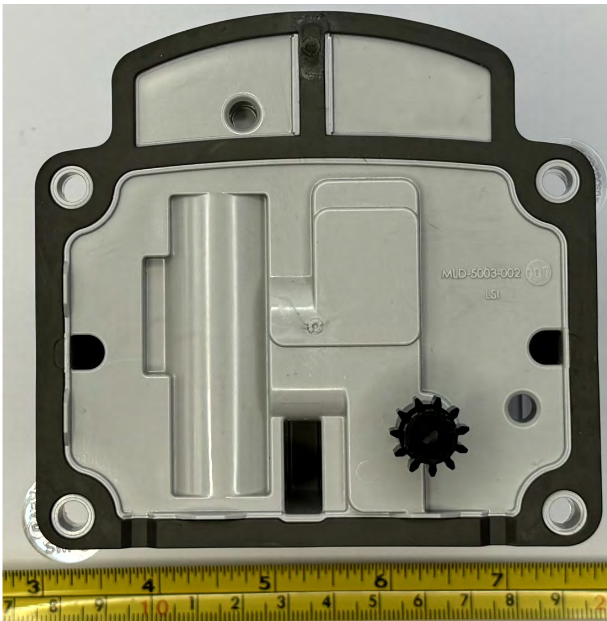
Figure 3.4: ERG-5600-002 External Back
