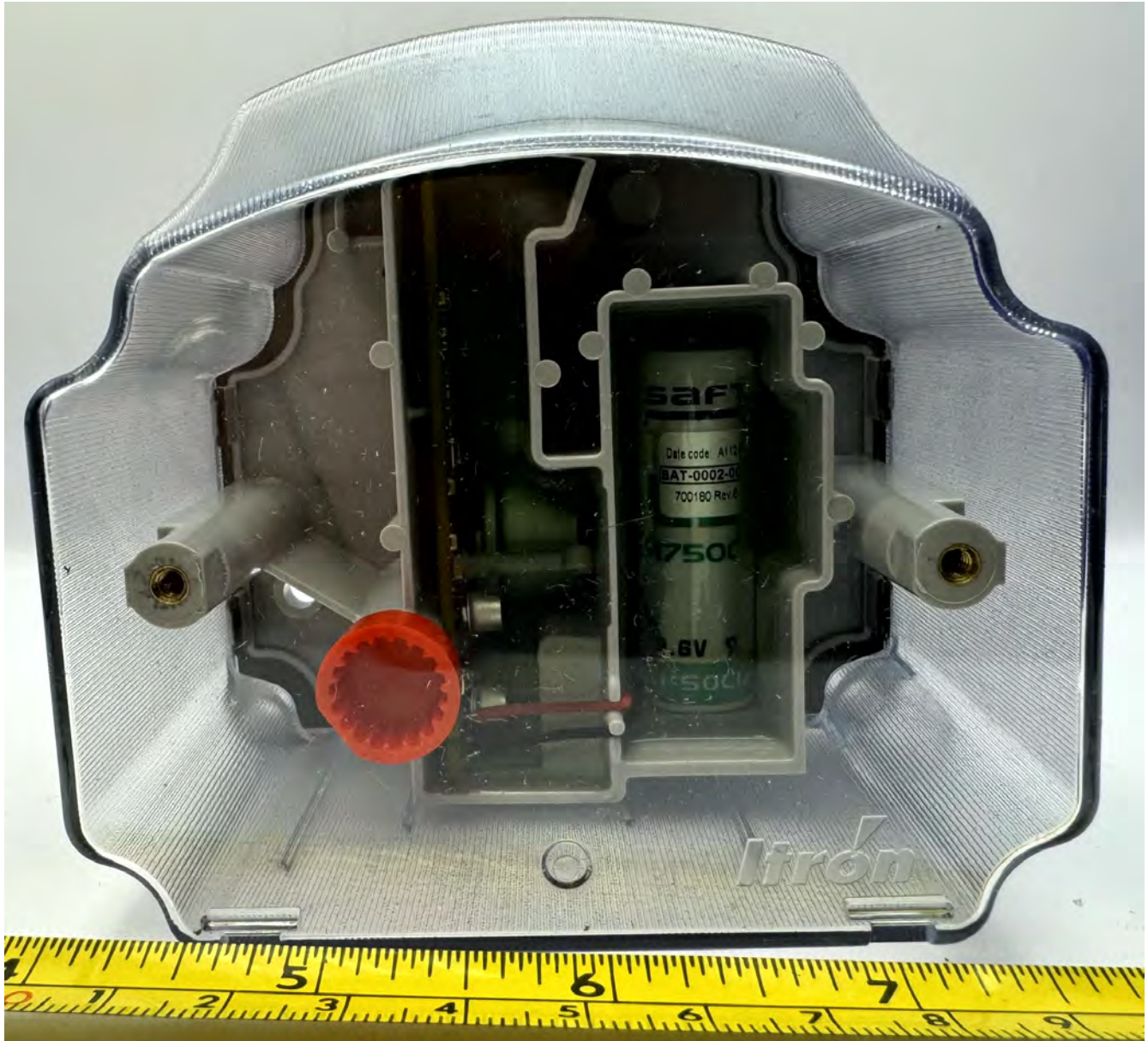
Figure 5.1: ERG-5600-004 External Front
