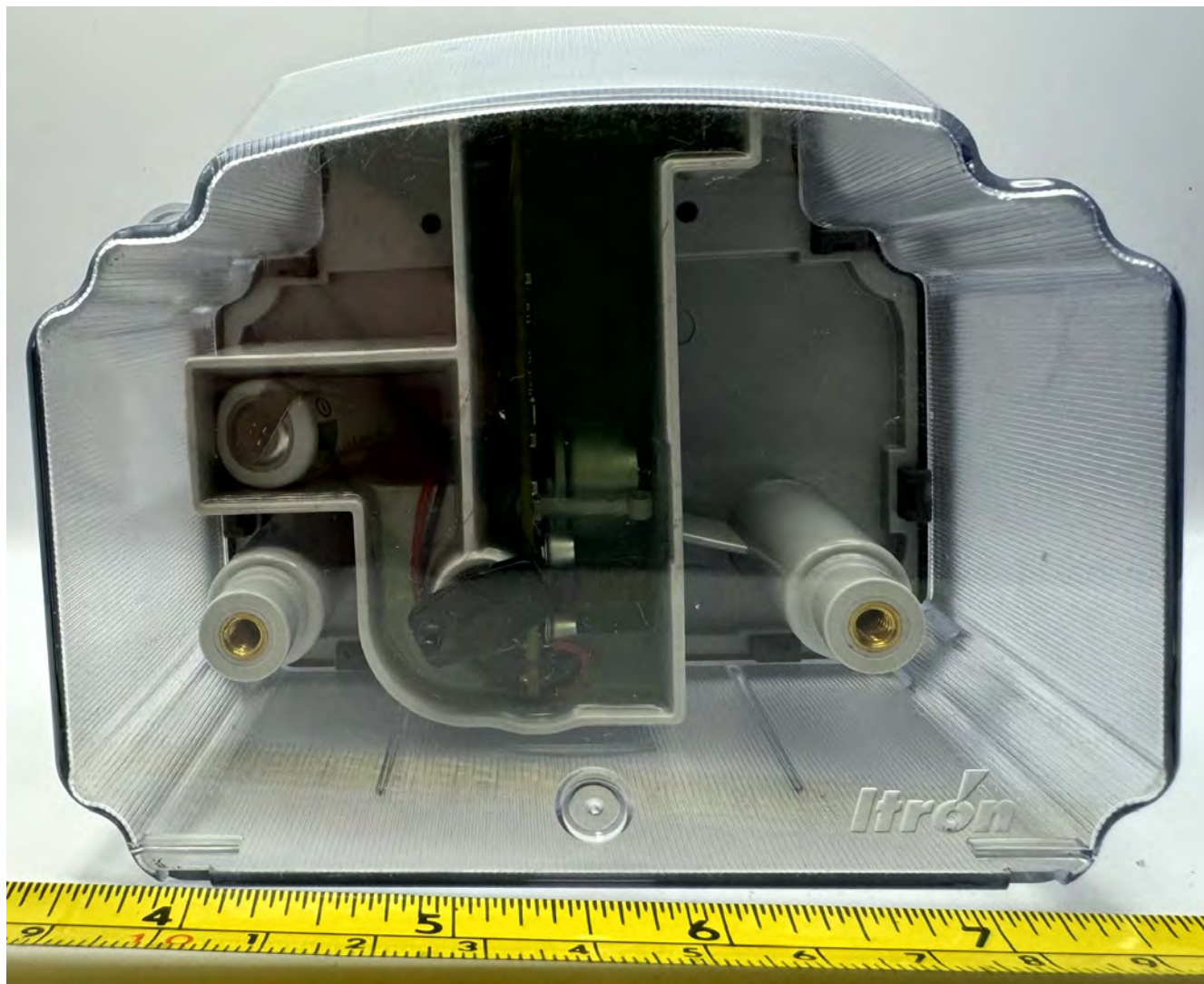
Figure 6.1: ERG-5600-009 External Front
