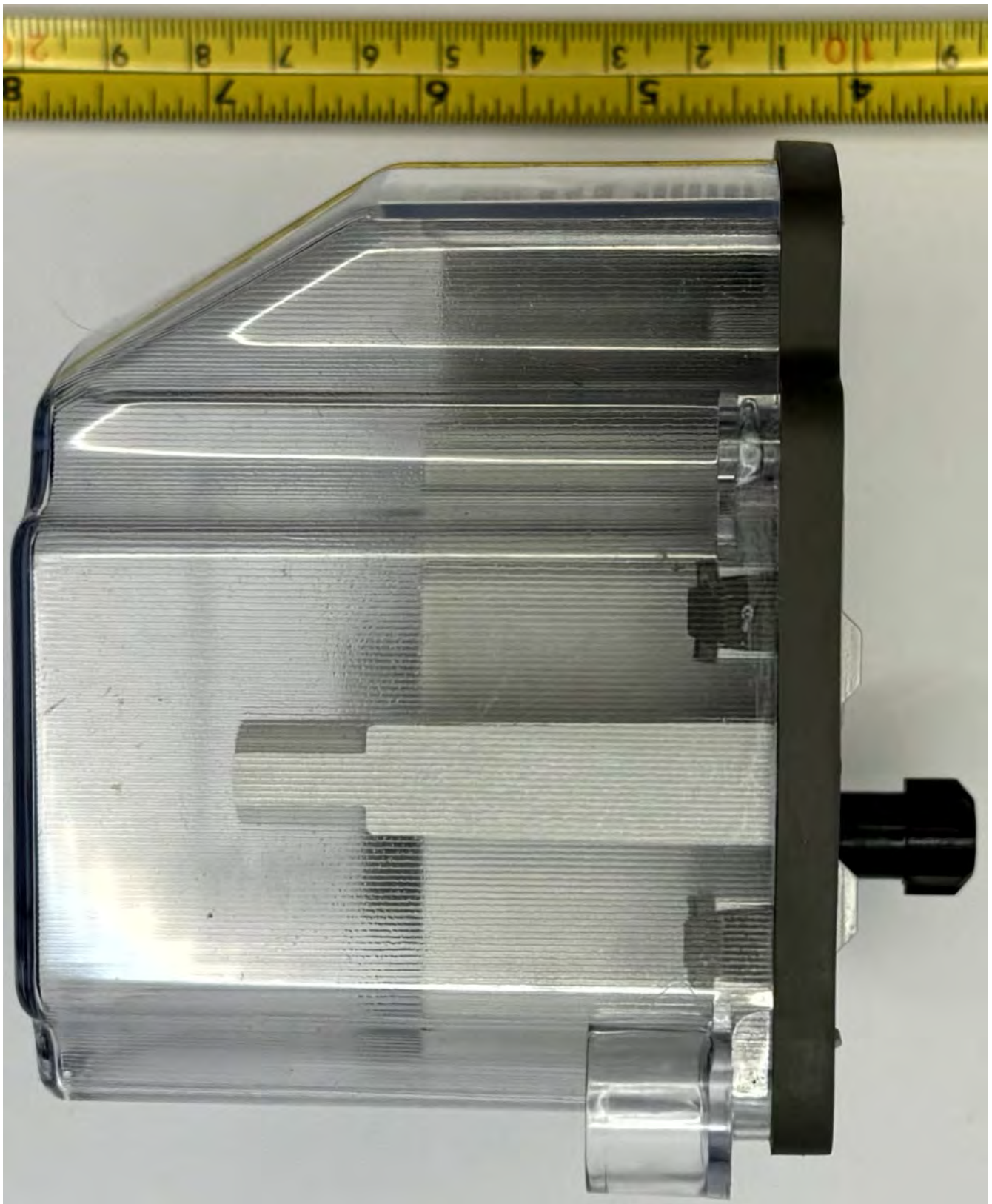
Figure 3.3: ERG-5600-002 External Right
