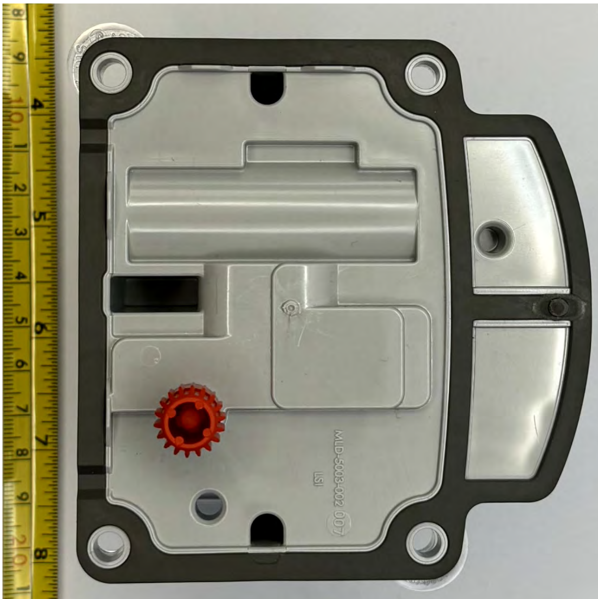
Figure 5.4: ERG-5600-004 External Back
