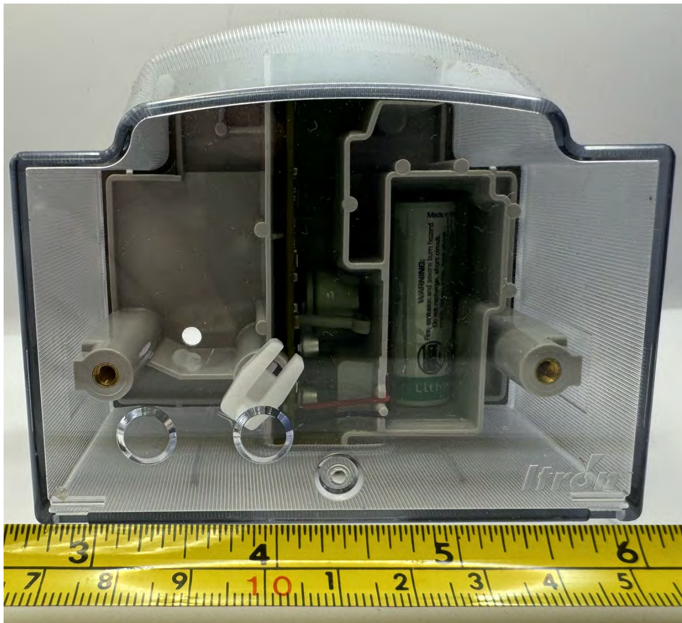
Figure 2.1: ERG-5600-001 External Front
