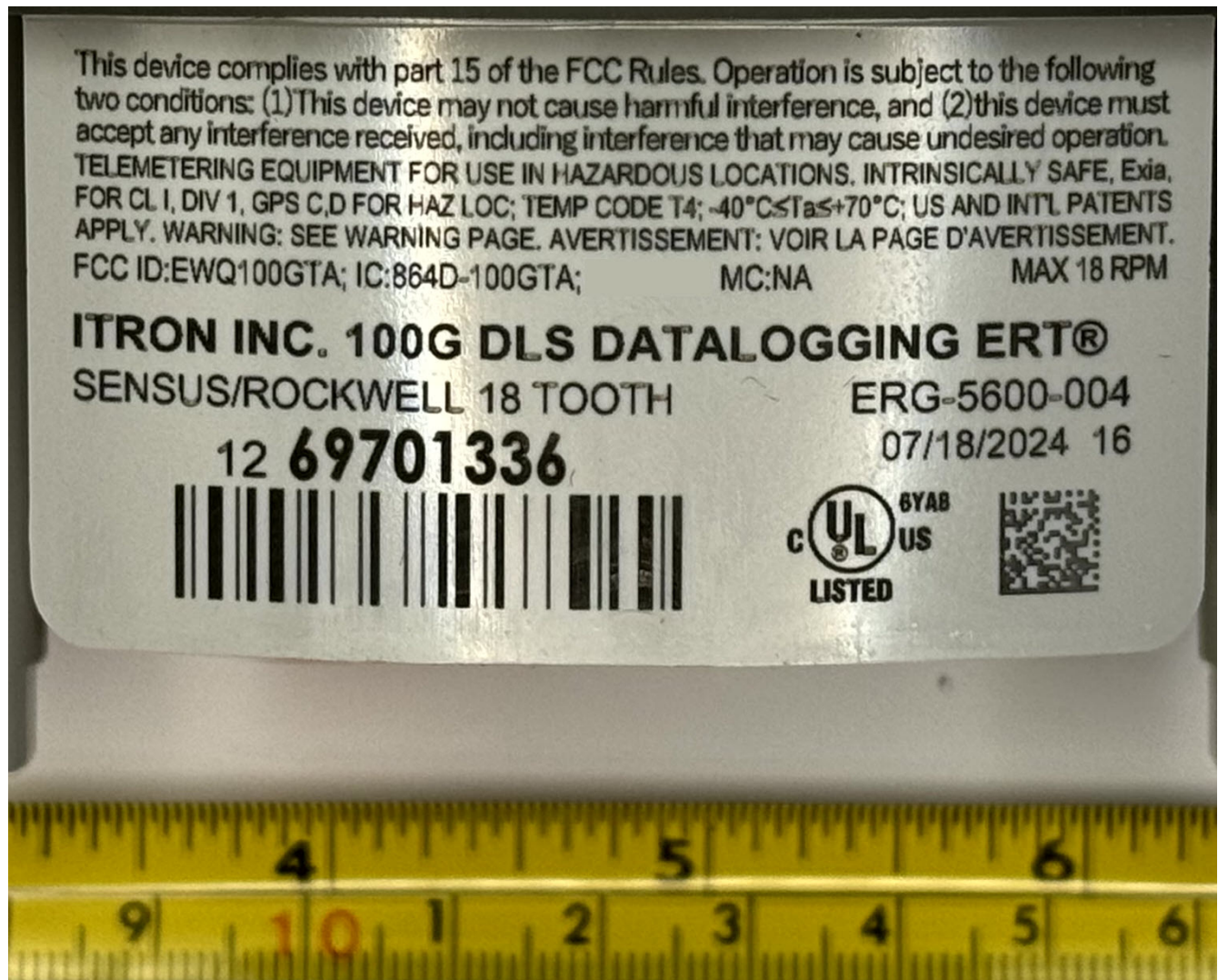
Figure 5.1: ERG-5600-004 Label
