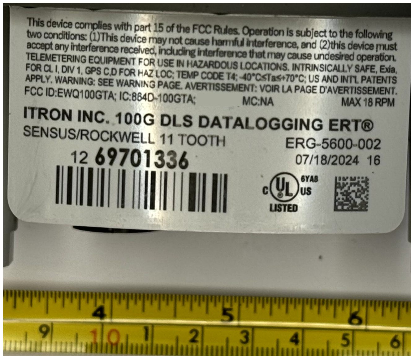
Figure 3.1: ERG-5600-002 Label
