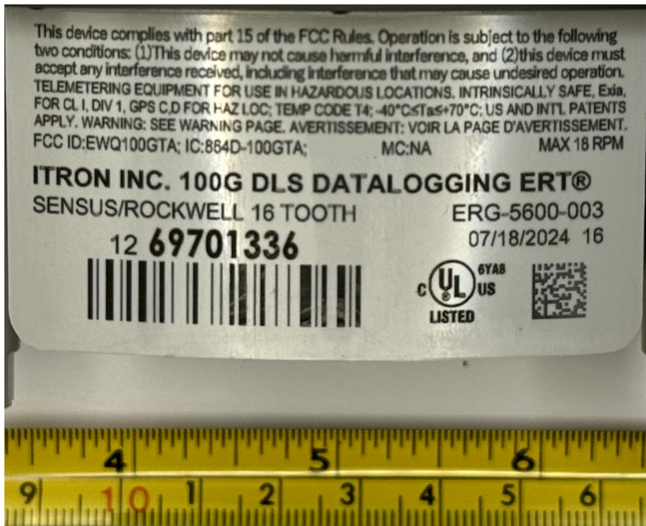
Figure 4.1: ERG-5600-003 Label
