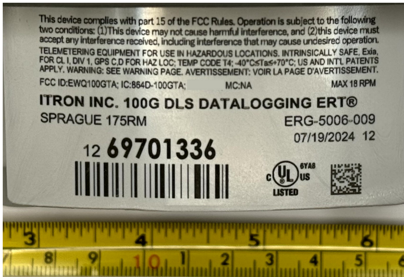
Figure 6.1: ERG-5600-009 Label
