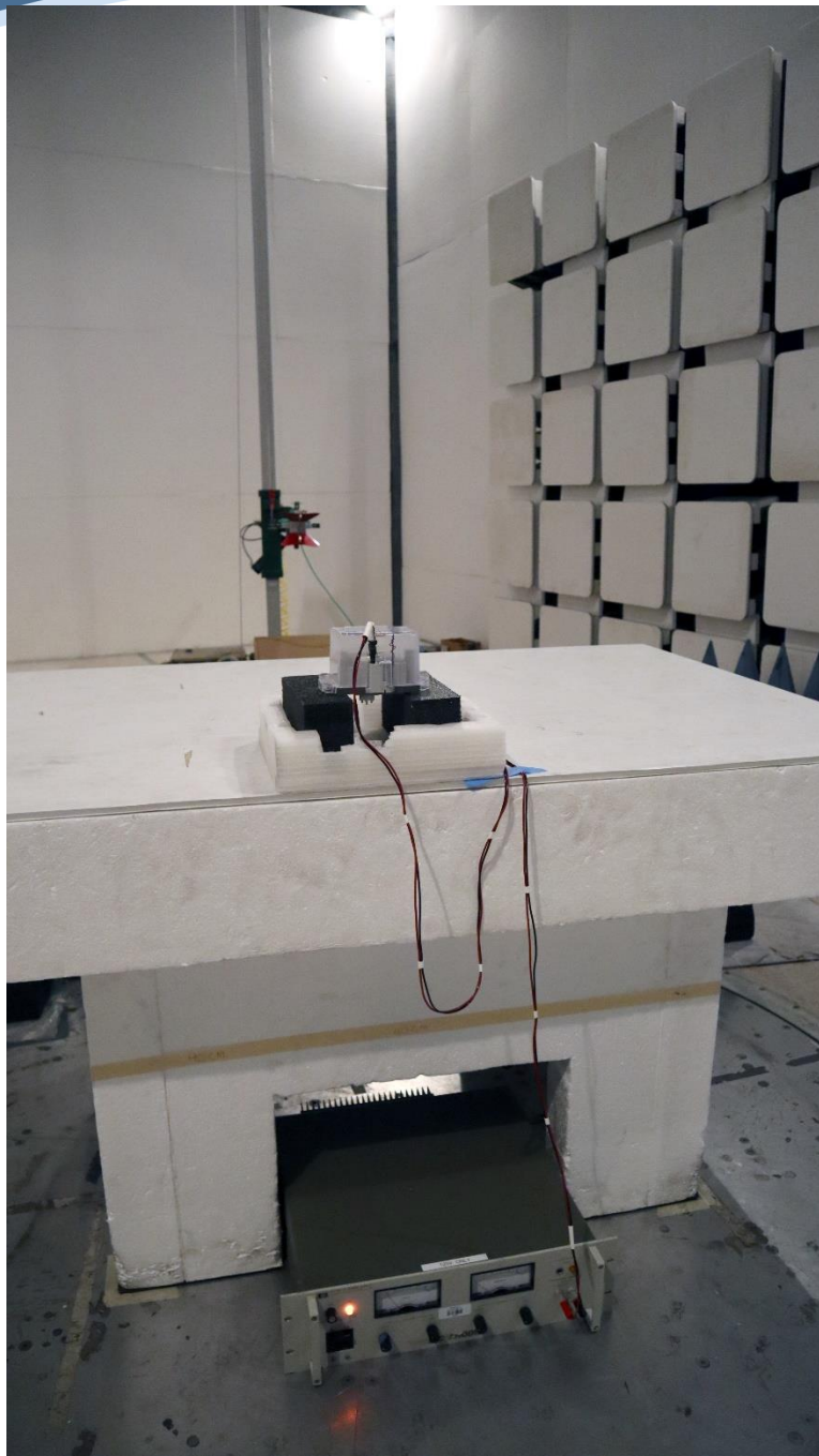
Digital Emission ERG-5600-001, 1-18GHz Front
