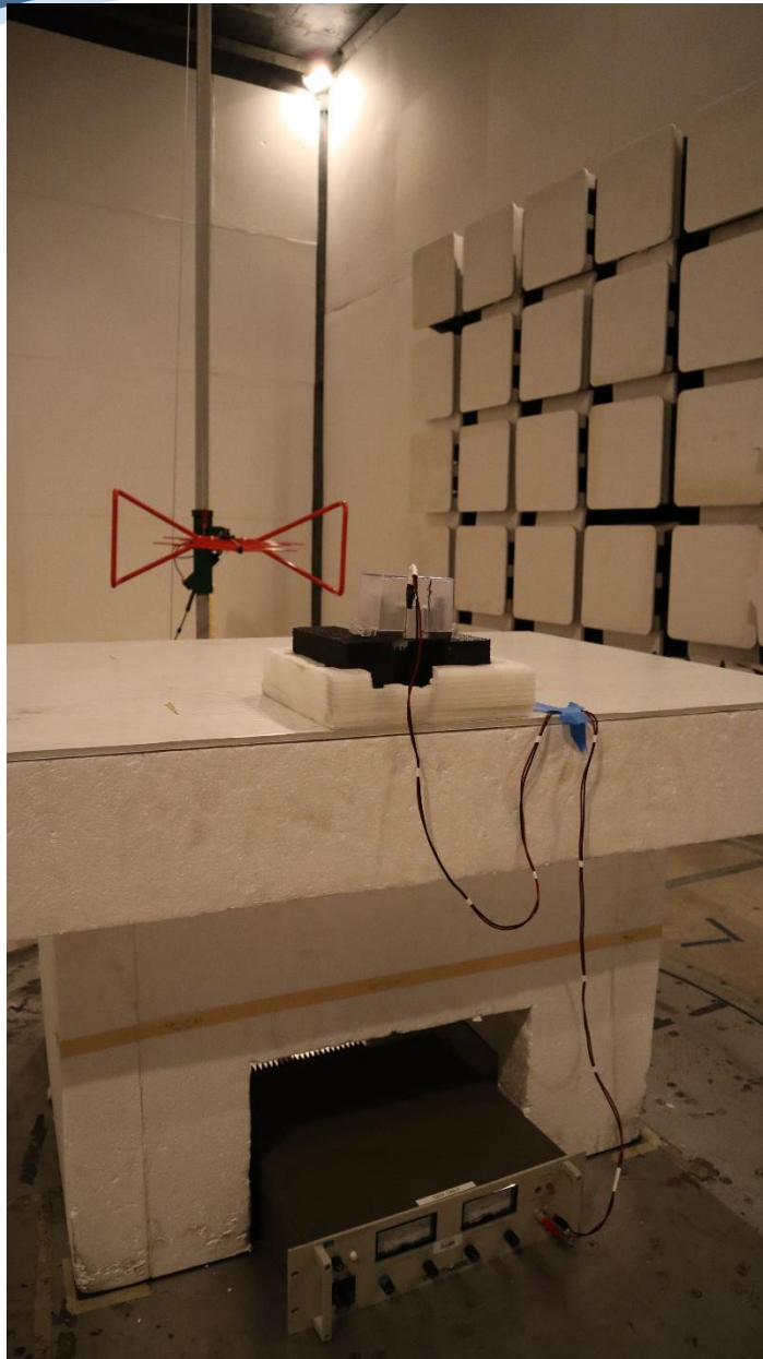
ERG-5600-001, 30MHz-1GHz front
