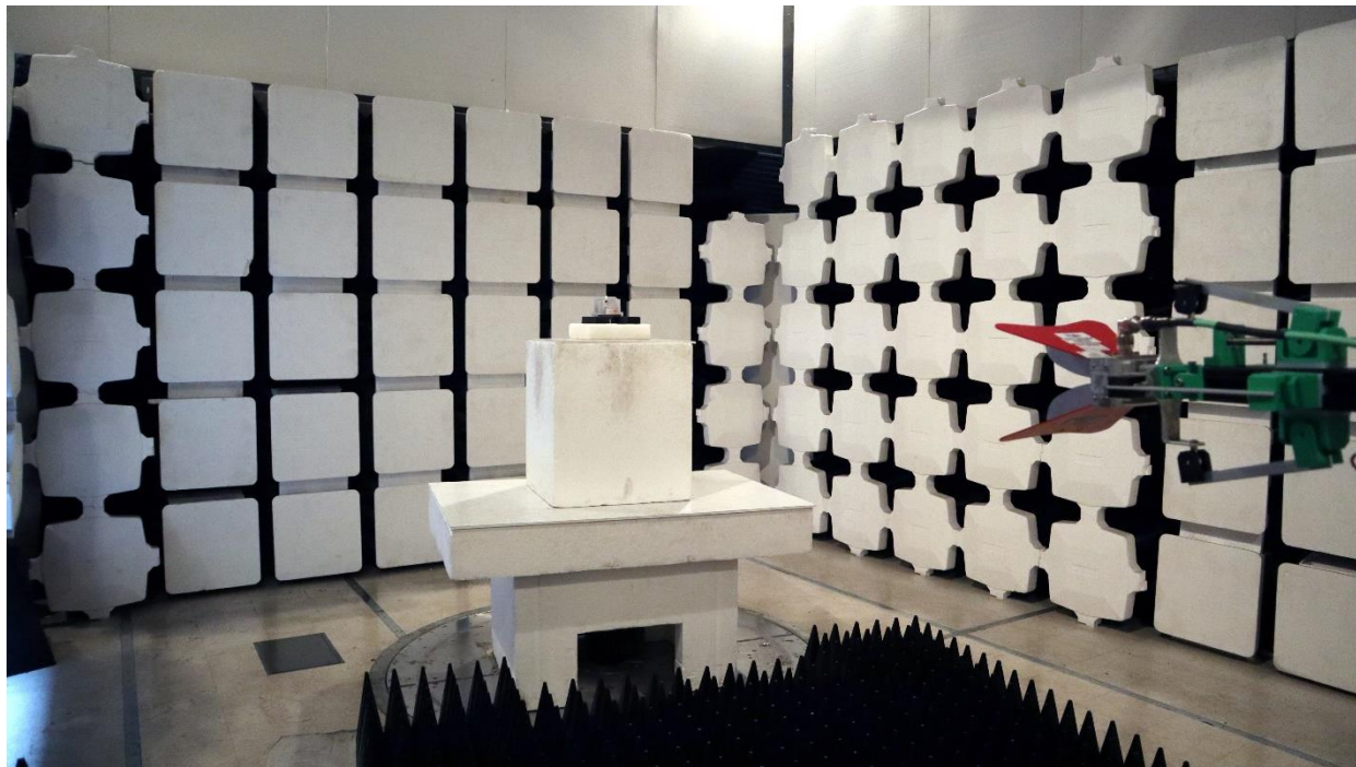
Spurious Emission ERG-5600-001, 1-18GHz Back
