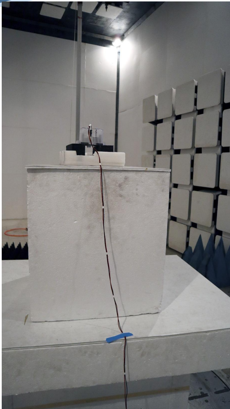
Spurious Emission ERG-5600-001, 1-18GHz Front
