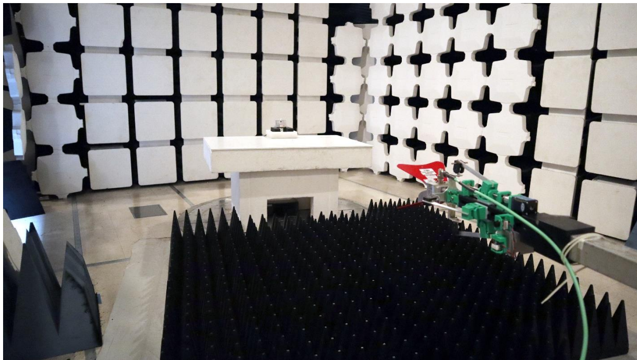
Digital Emission ERG-5600-001, 1-18GHz Back
