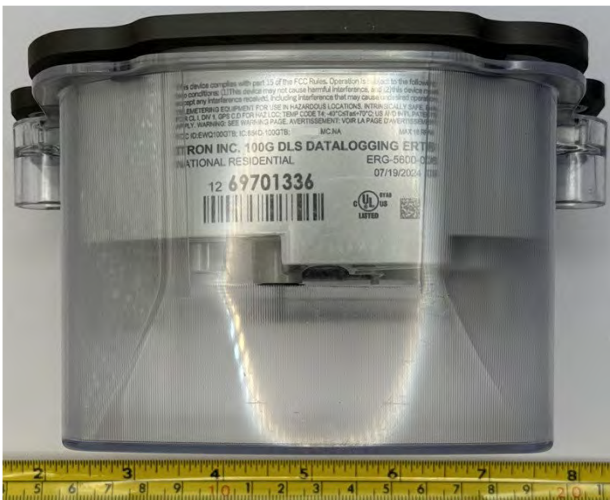
Figure 3.5: ERG-5600-006 External Top
