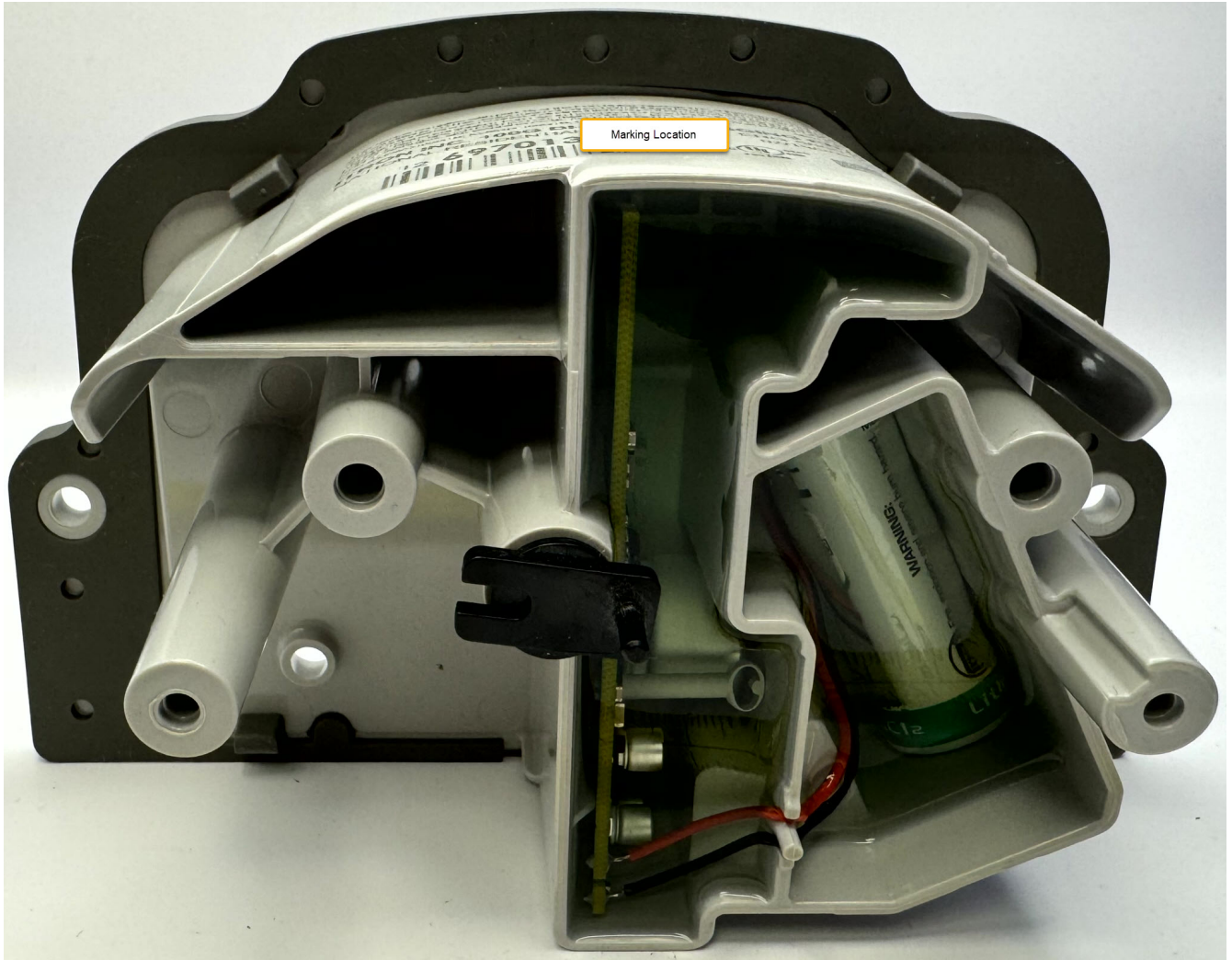
Figure 3.2: ERG-5600-006 Label Location
