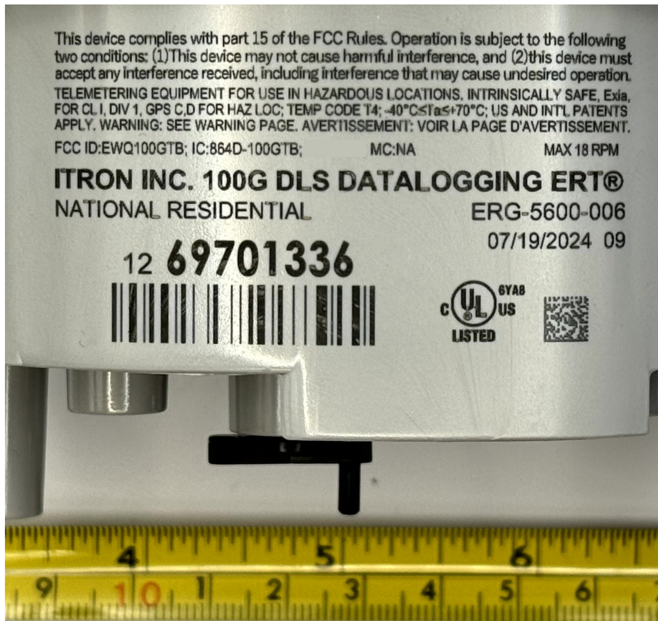
Figure 3.1: ERG-5600-006 Label
