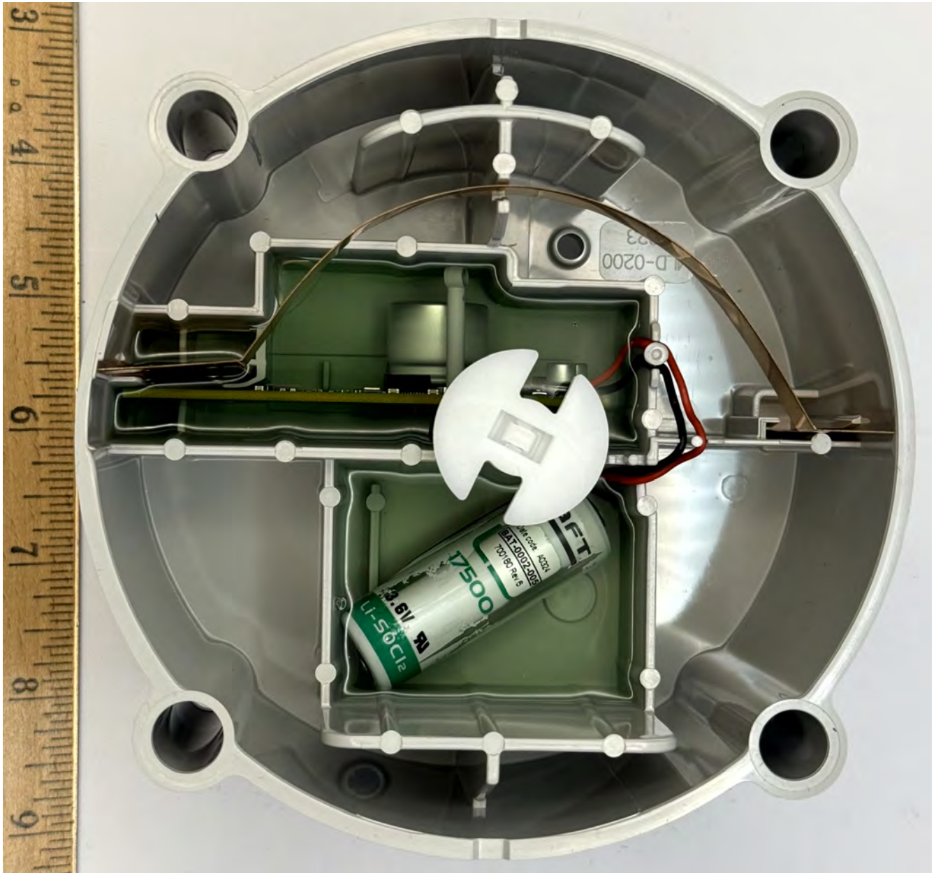
Figure 2.6: ERG-5600-007 External Bottom
