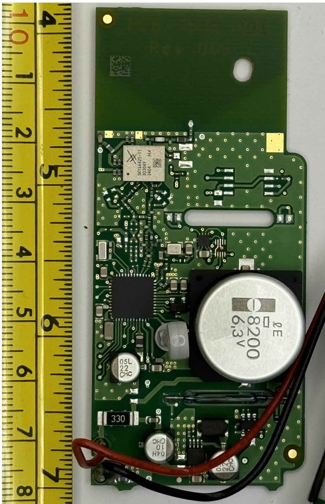
Figure 2.1: PCB Front
