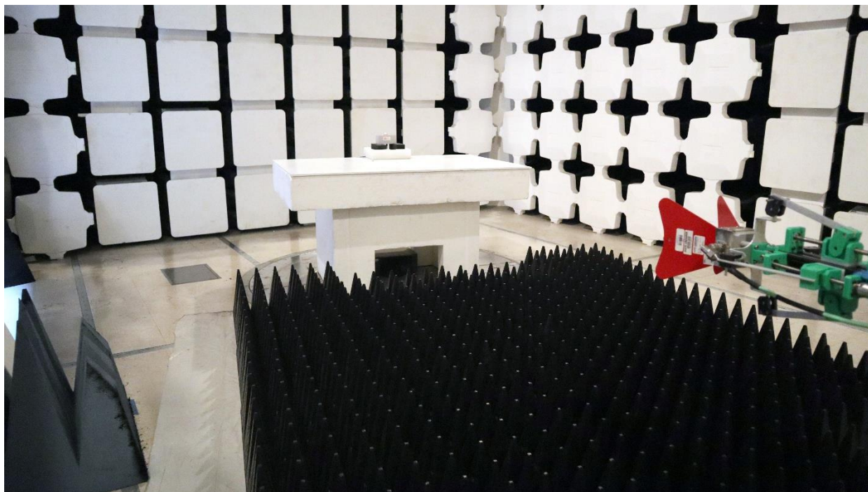
Digital Emissions ERG-5600-008, 1-18GHz Back, Horizontal
