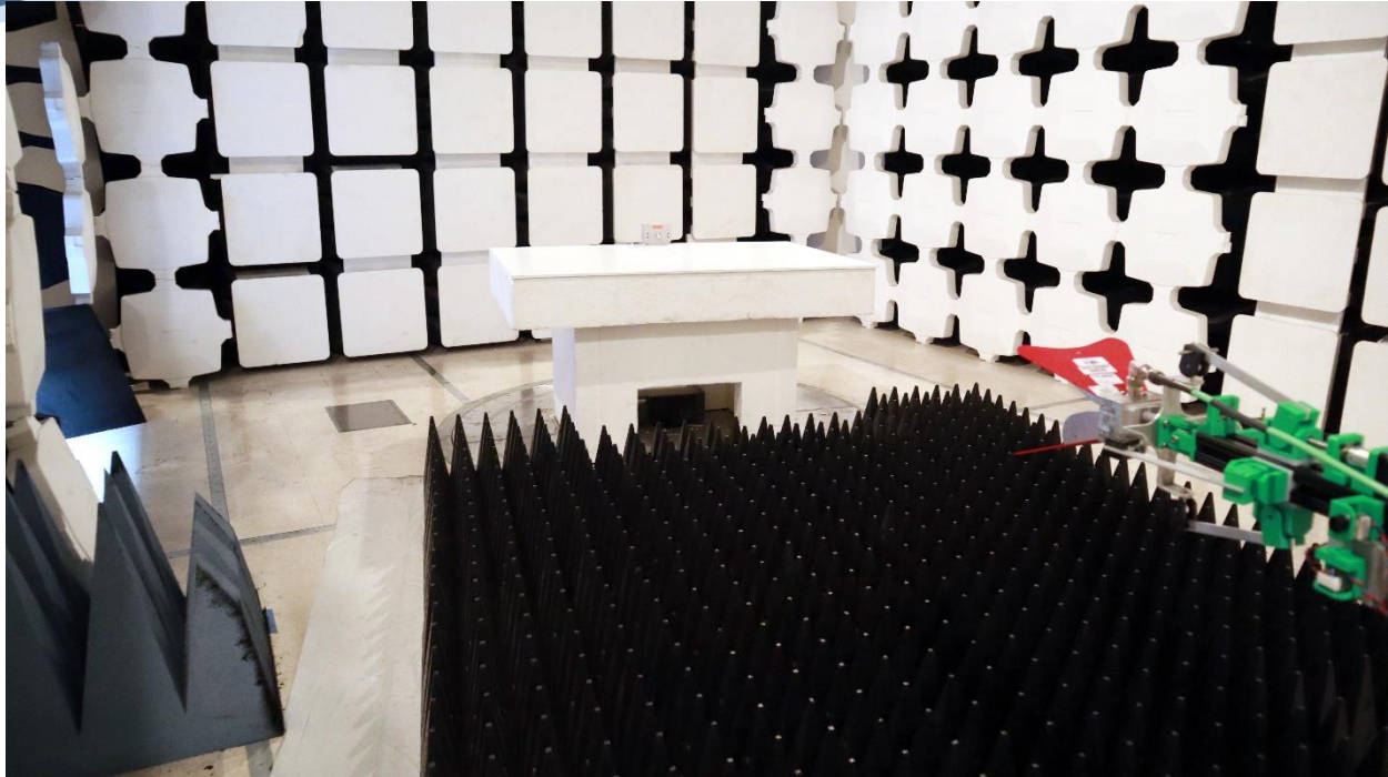
Digital Emissions ERG-5600-008, 1-18GHz Back, Power Cable Down
