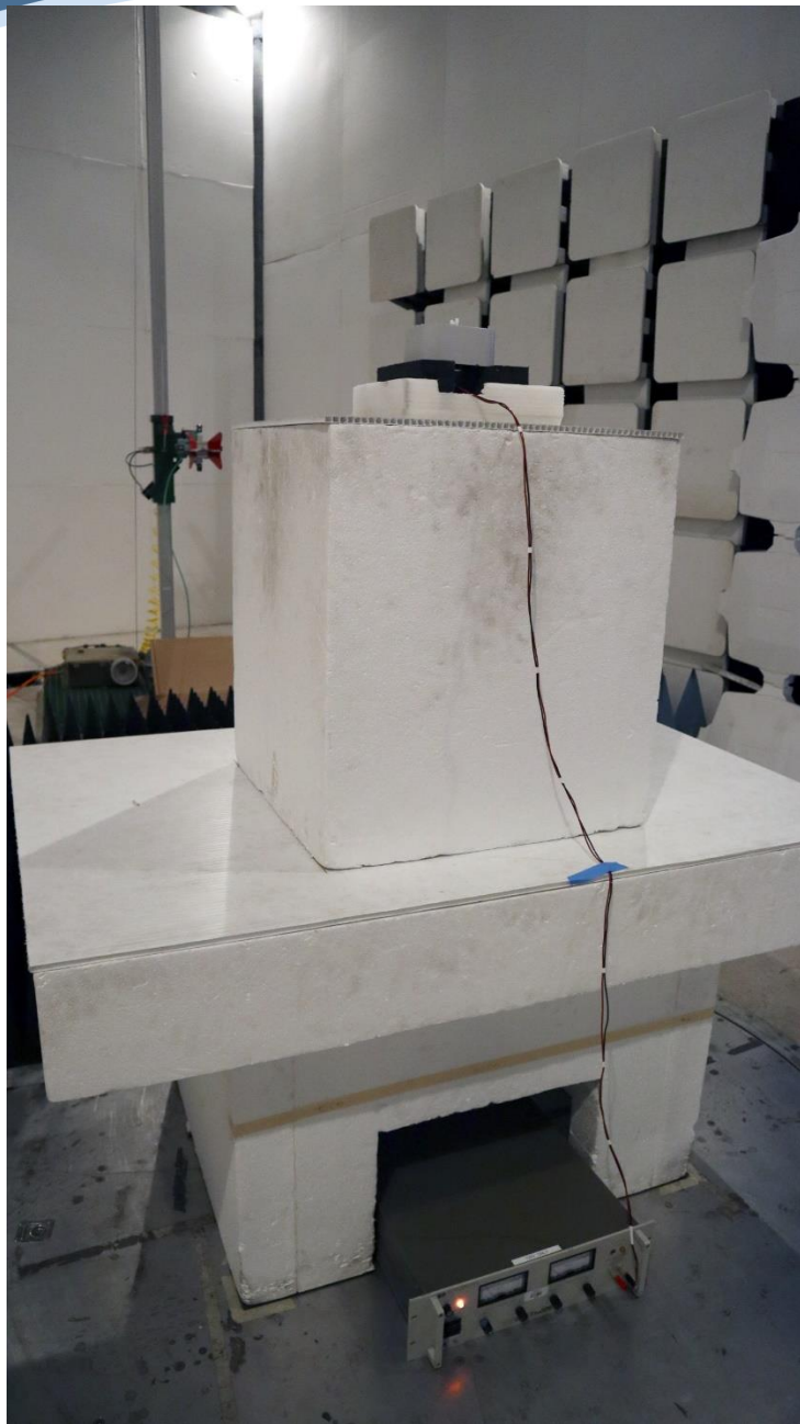
Spurious Emissions ERG-5600-008, 1-18GHz Front, Horizontal
