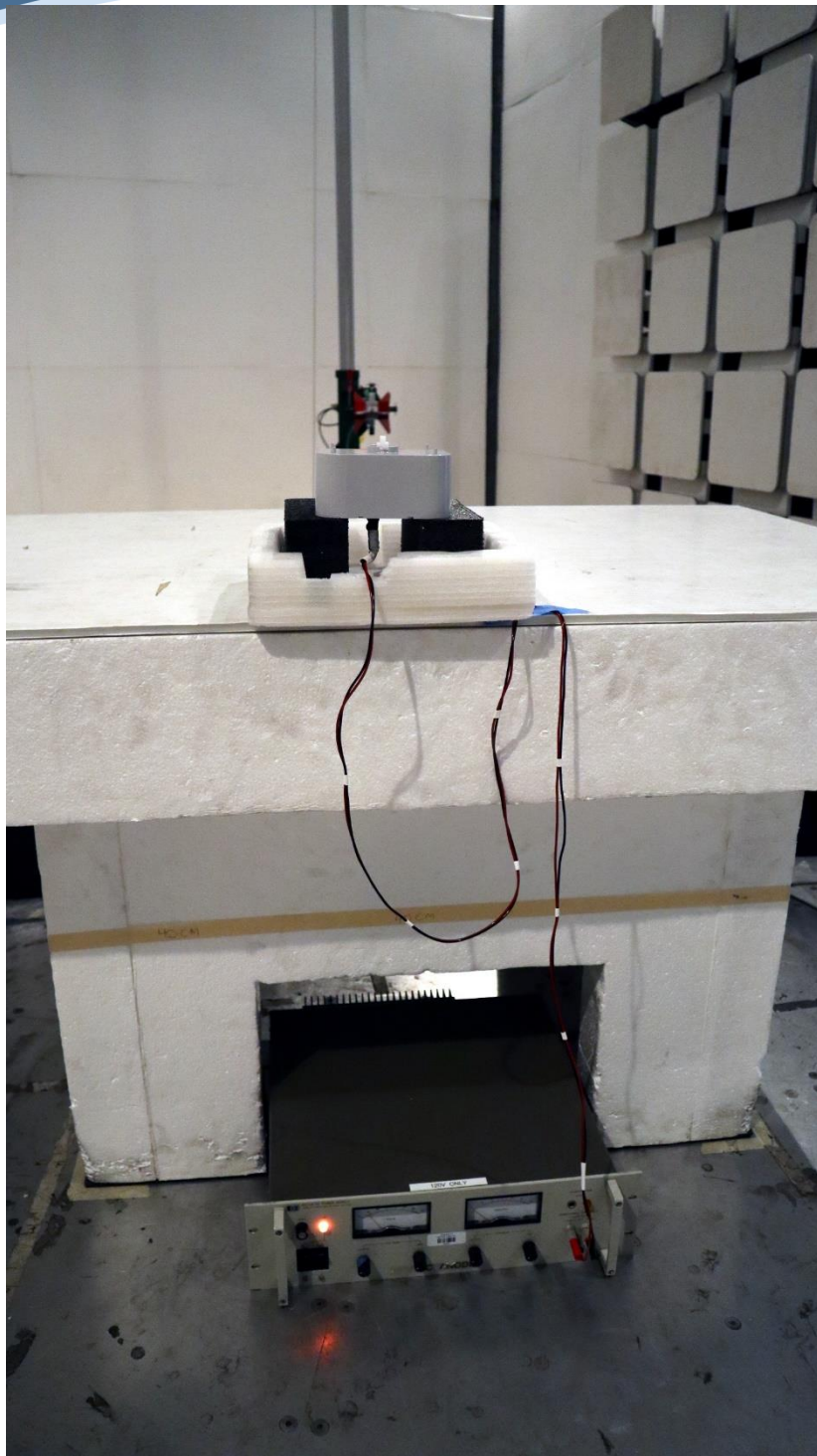
Digital Emissions ERG-5600-008, 1-18GHz Front, Horizontal
