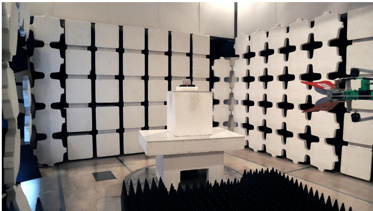
Spurious Emissions ERG-5600-008, 1-18G Back, Power Cable Up
