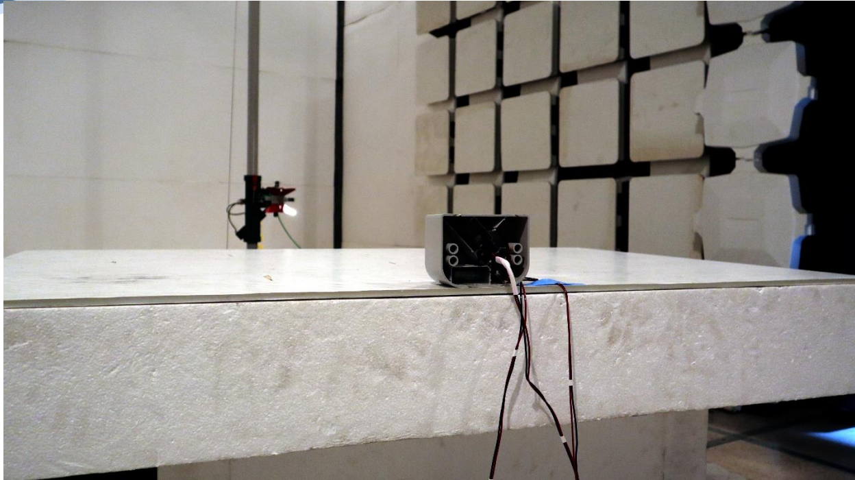
Digital Emissions ERG-5600-008, 1-18GHz Front, Power Cable Down
