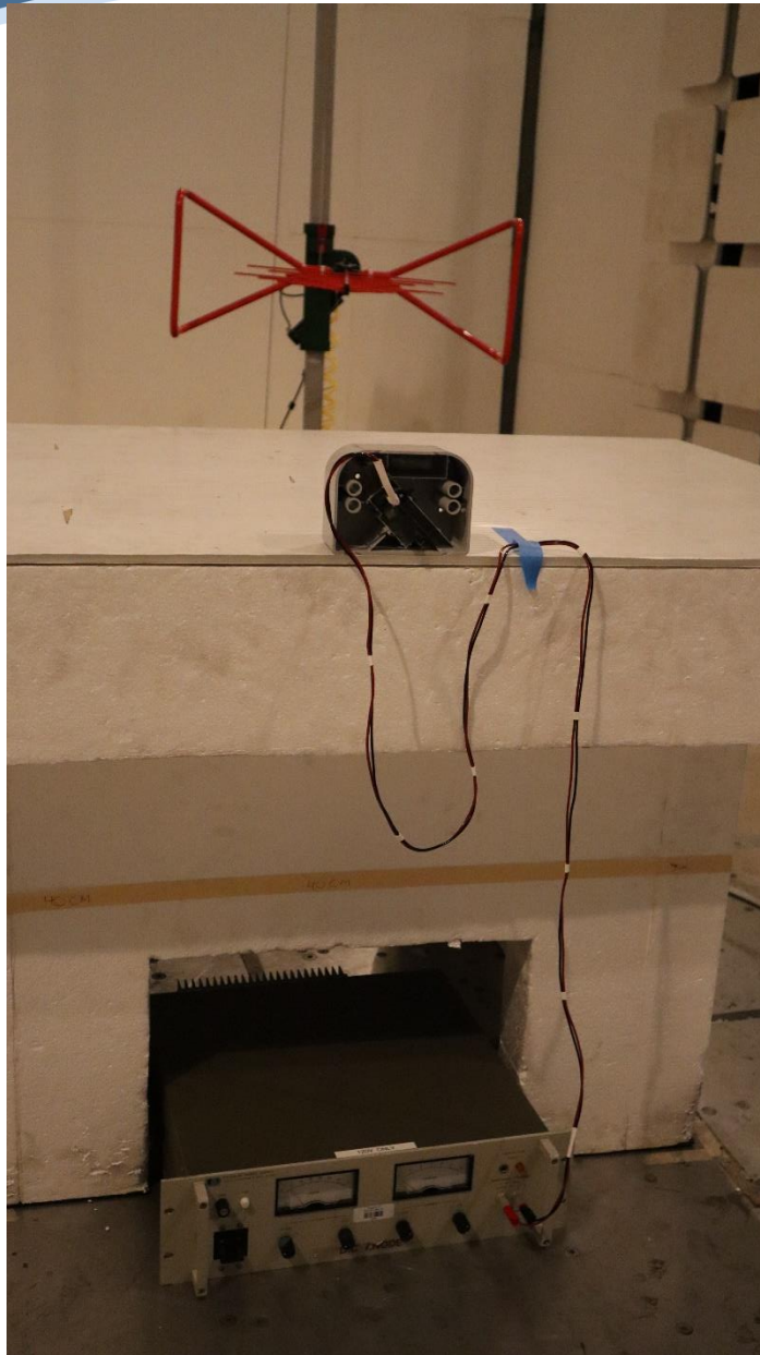
ERG-5600-008, 30MHz-1GHz Front, Power Cable Up
