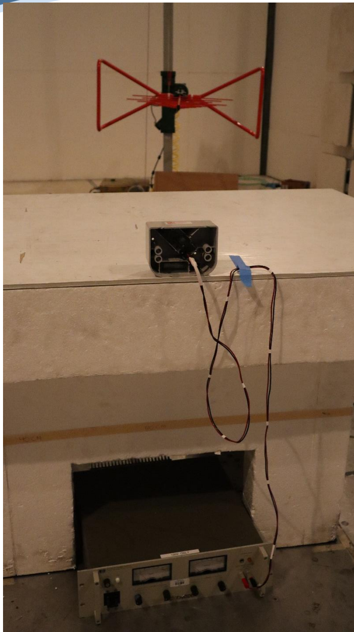
ERG-5600-008, 30MHz-1GHz Front, Power Cable Down
