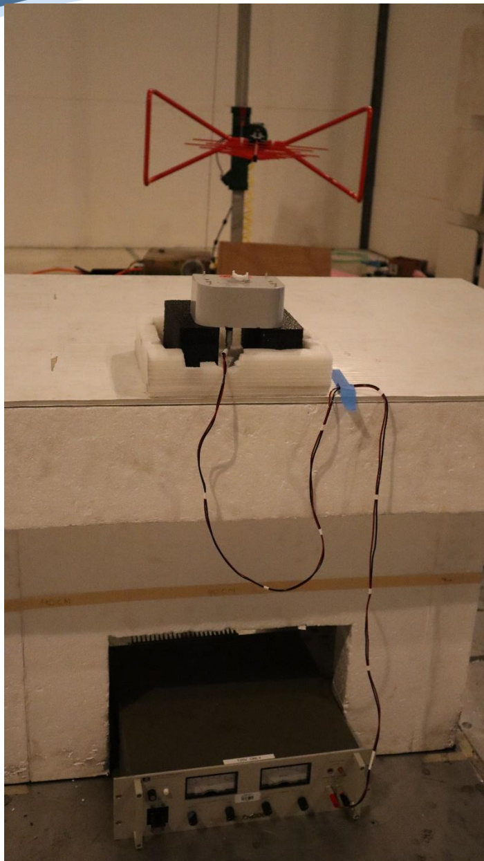
ERG-5600-008, 30MHz-1GHz Front, Horizontal
