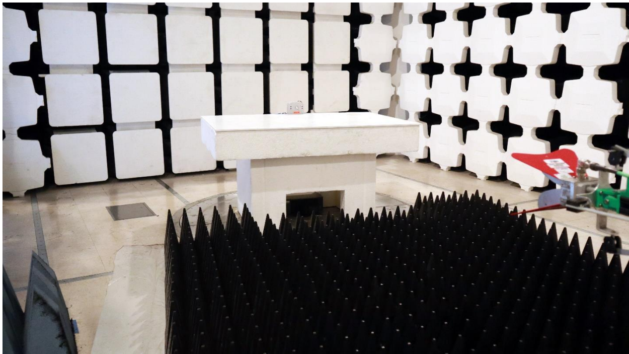
Digital Emissions ERG-5600-008, 1-18GHz Back, Power Cable Up
