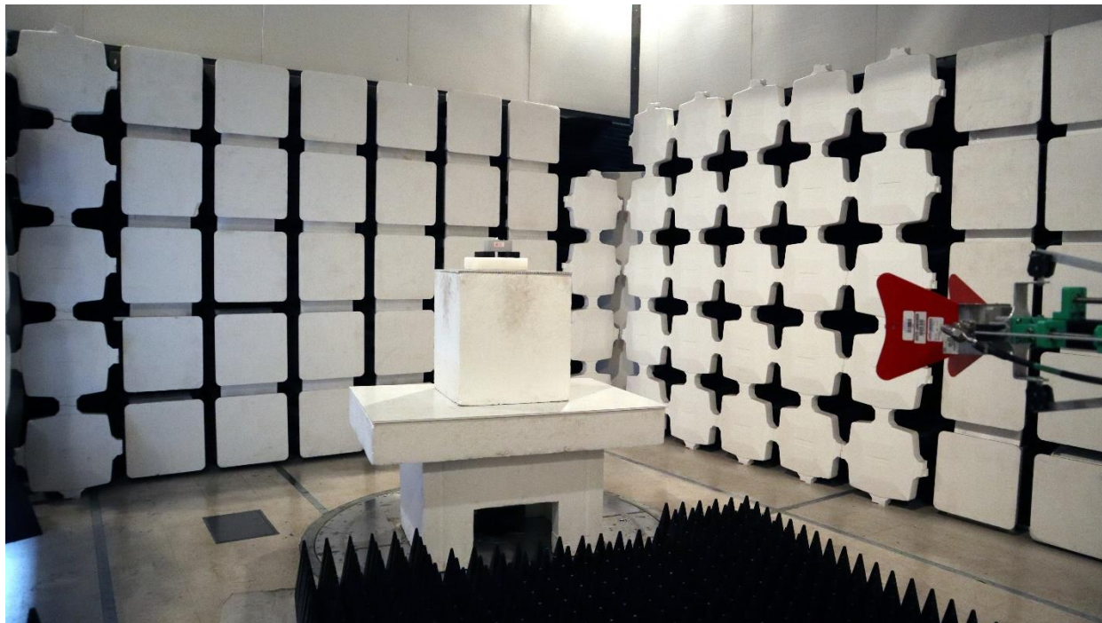
Spurious Emissions ERG-5600-008, 1-18GHz Back, Horizontal
