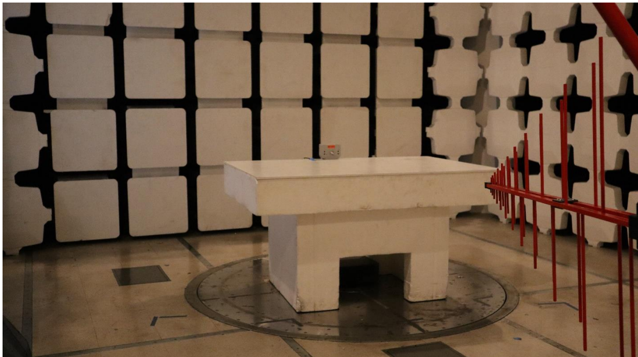
ERG-5600-008, 30MHz-1GHz Back, Power Cable Down
