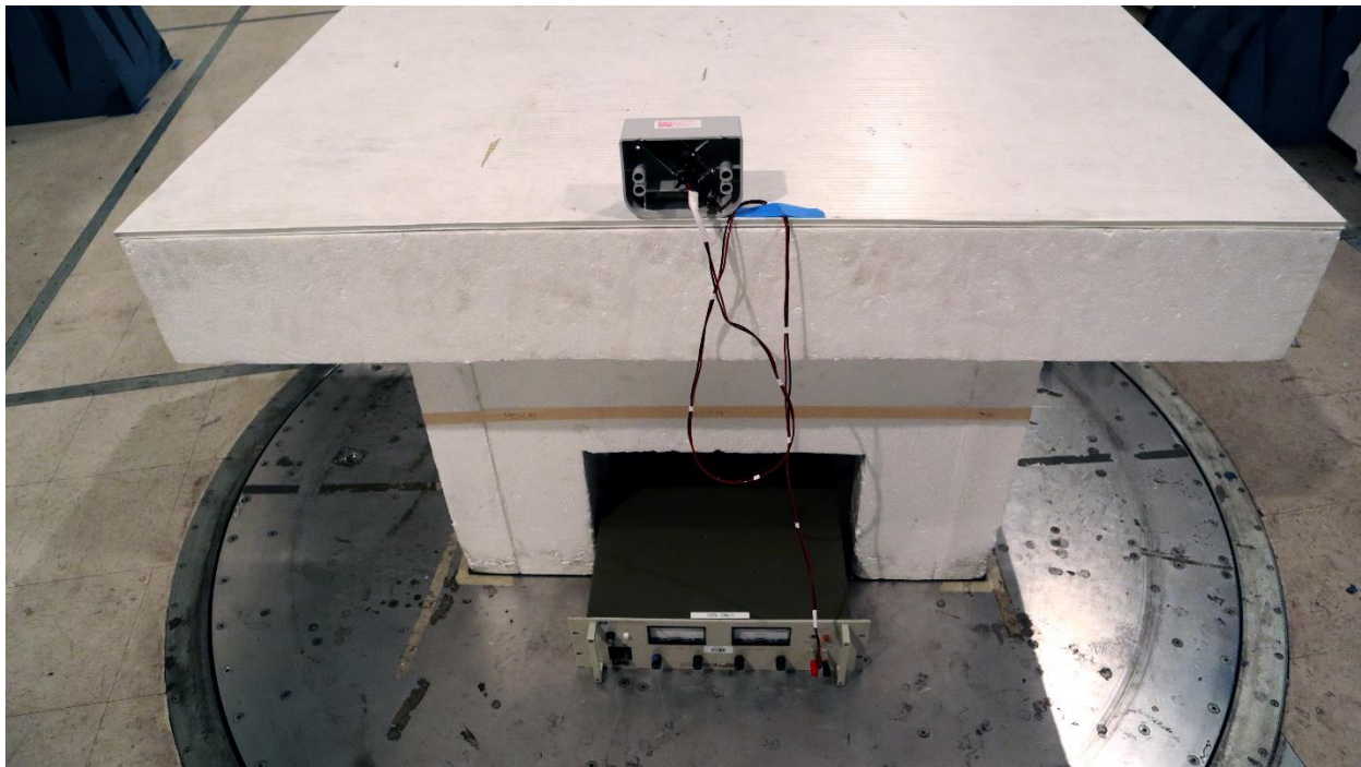
Digital Emissions ERG-5600-008, 1-18GHz Front, Power Cable Down
