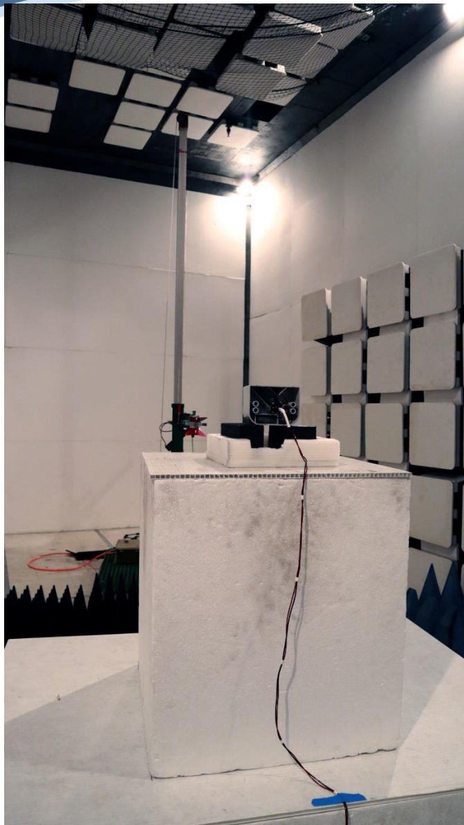
Spurious Emissions ERG-5600-008, 1-18GHz Front, Power Cable Down
