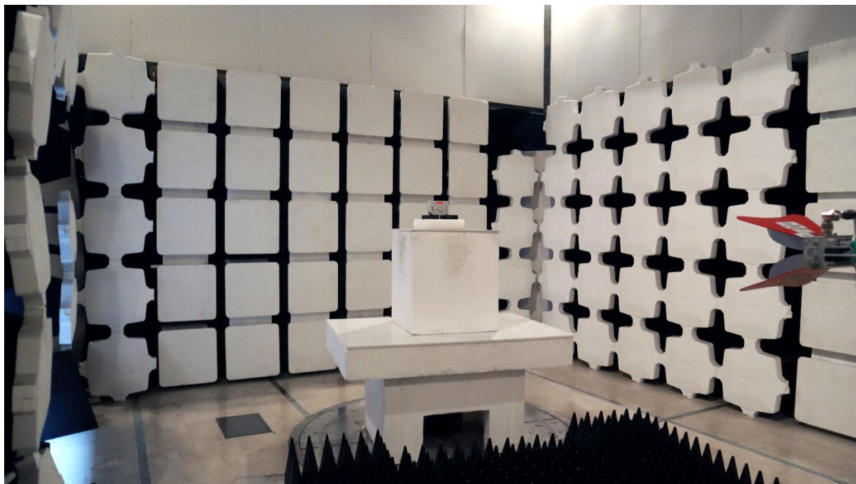
Spurious Emissions ERG-5600-008, 1-18GHz Back, Power Cable Down
