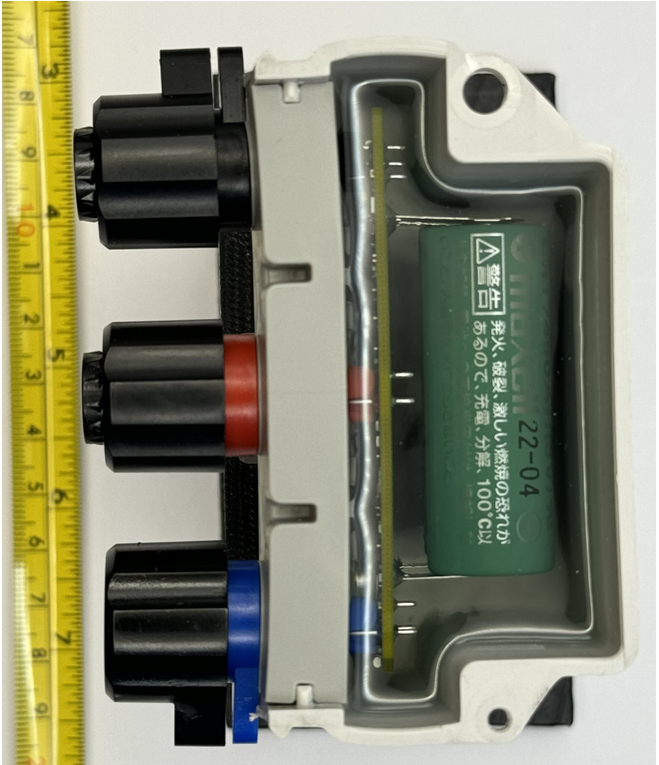
Figure 2.13: ERW-1350-001 External Bottom
