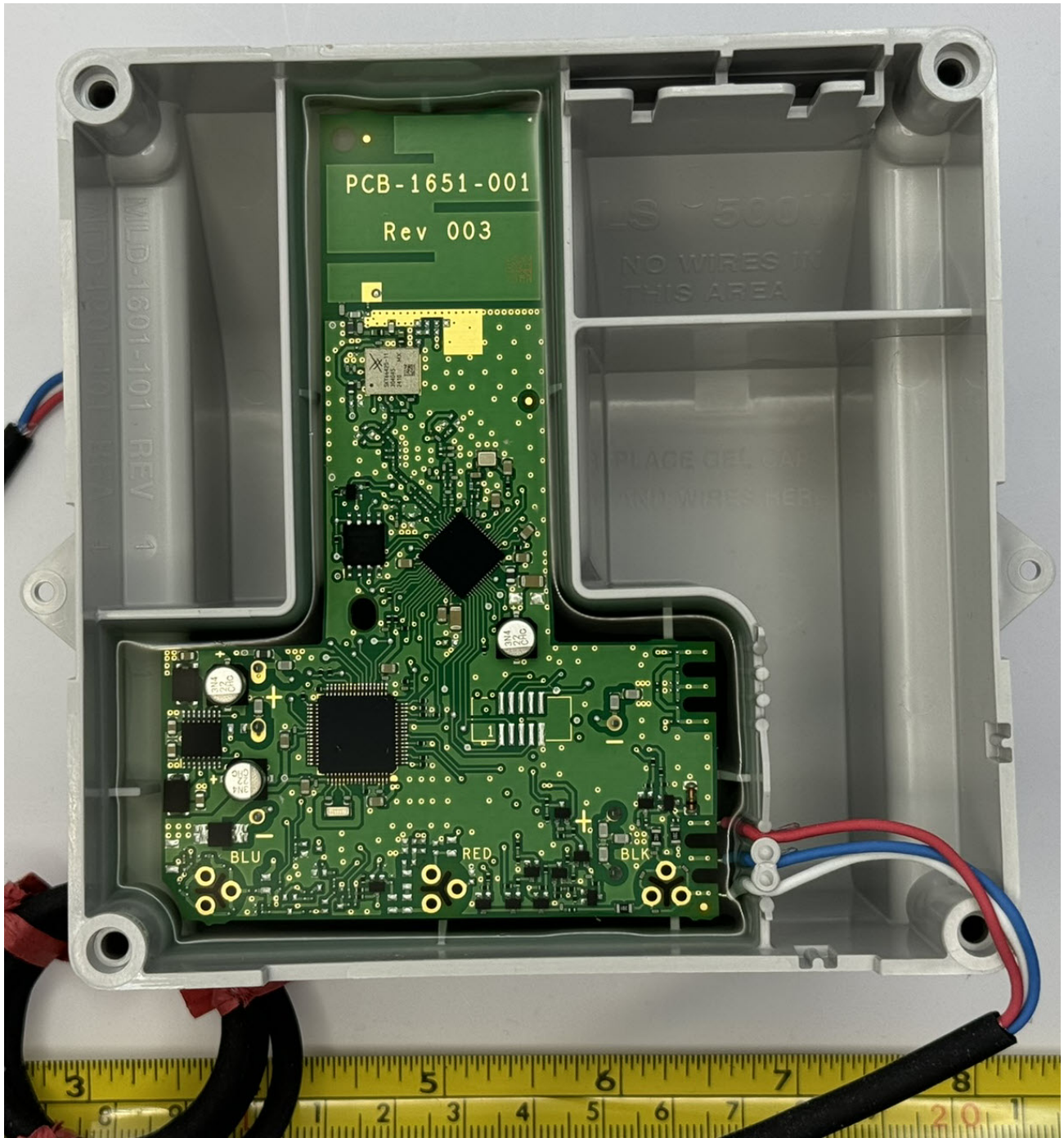
Figure 2.5: ERG-5600-501 External Back Plate Off
