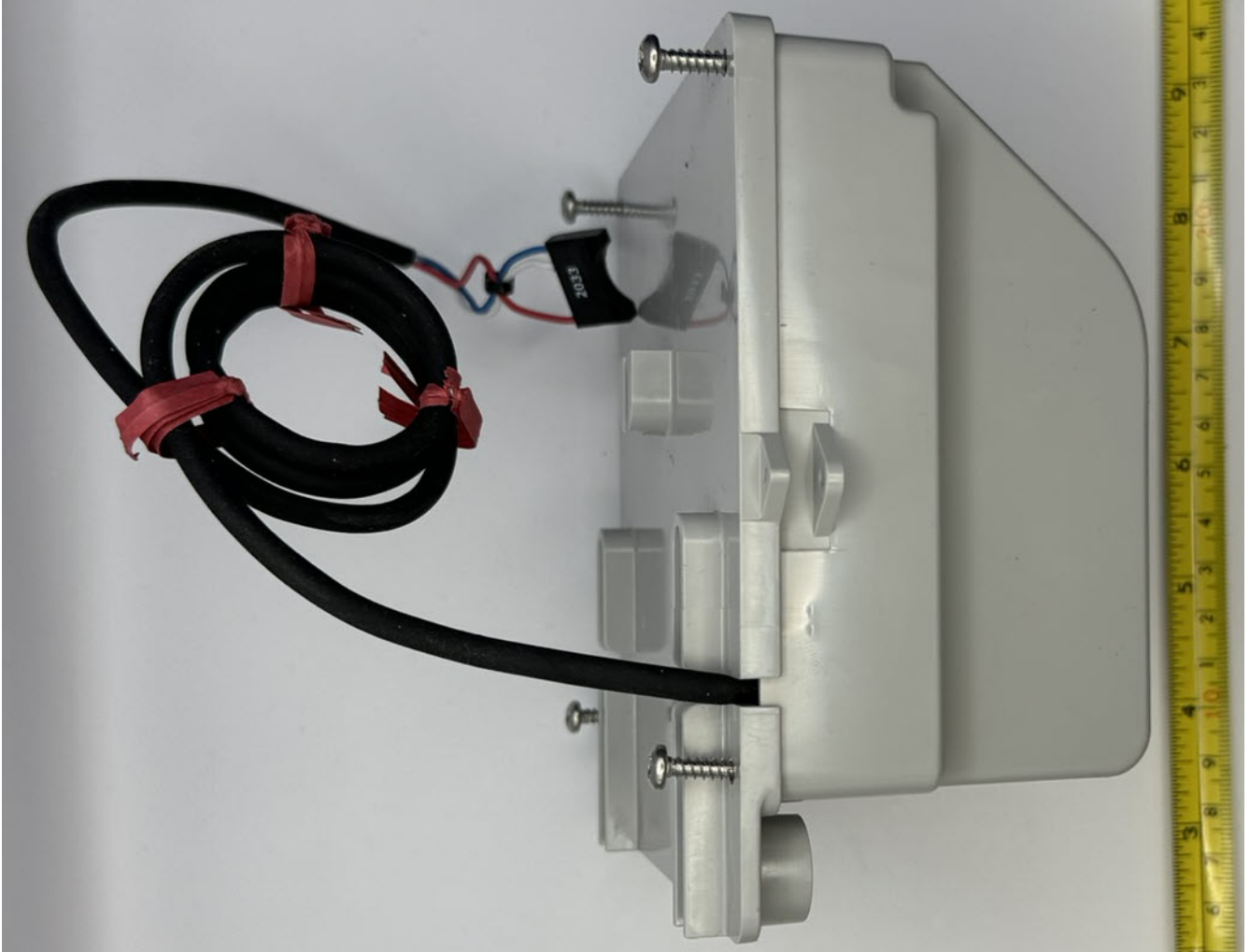
Figure 2.2: ERG-5600-501 External Left
