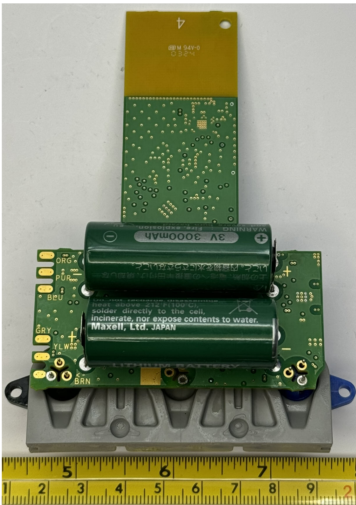
Figure 2.5: Pit 2-Battery, 2-Port - Back
