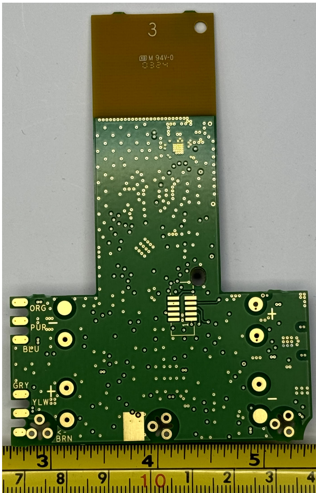
Figure 2.4: Pit & Remote Mount - PCB Back
