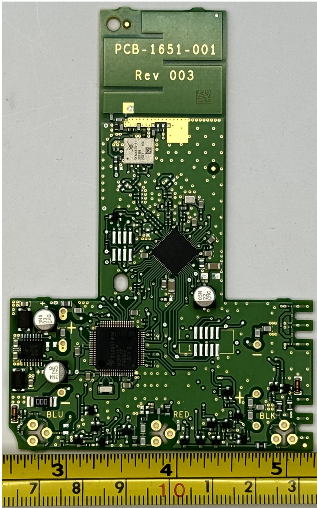
Figure 2.1: 100W Pit Mount - PCB Front
