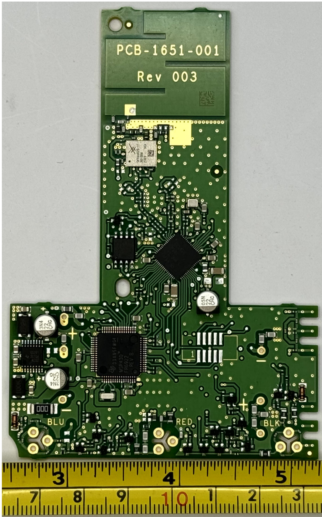
Figure 2.2: 500W Pit Mount - PCB Front
