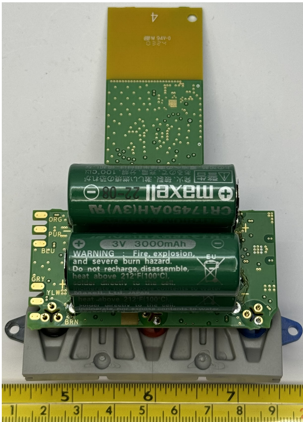
Figure 2.7: Pit 4-Battery, 3-Port - Back
