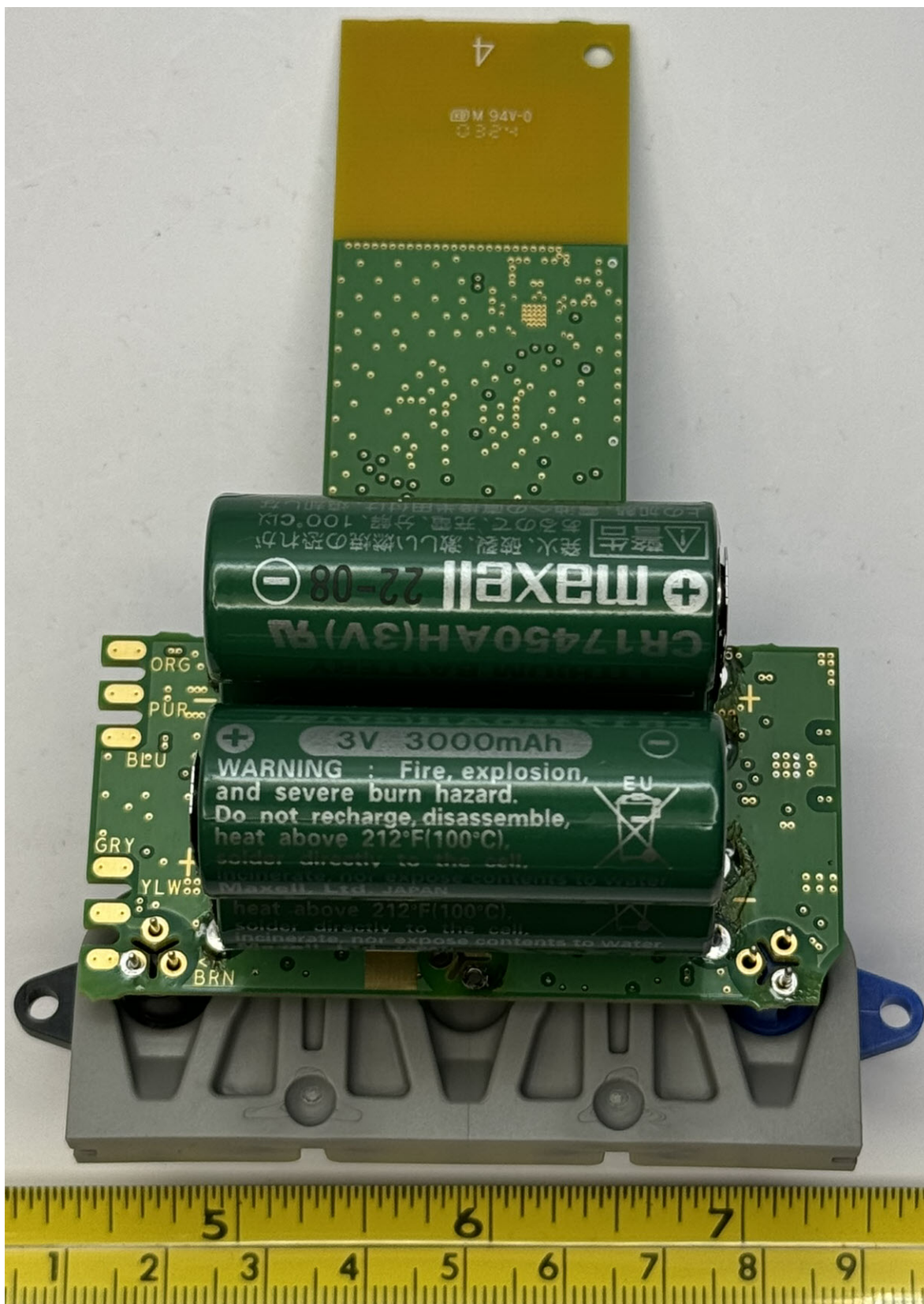
Figure 2.6: Pit 4-Battery, 2-Port - Back
