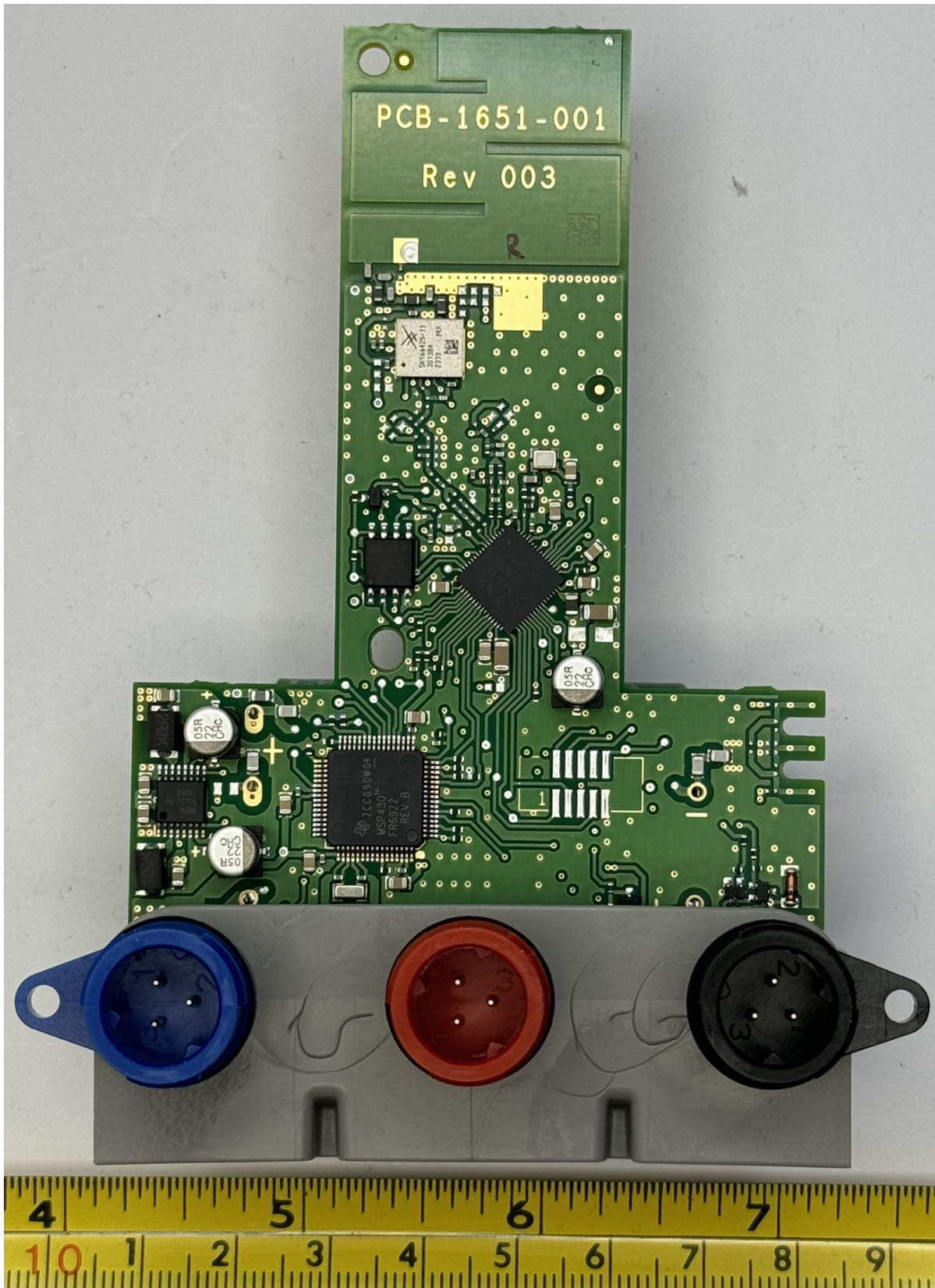
Figure 2.10: Pit 3-Port - Front
