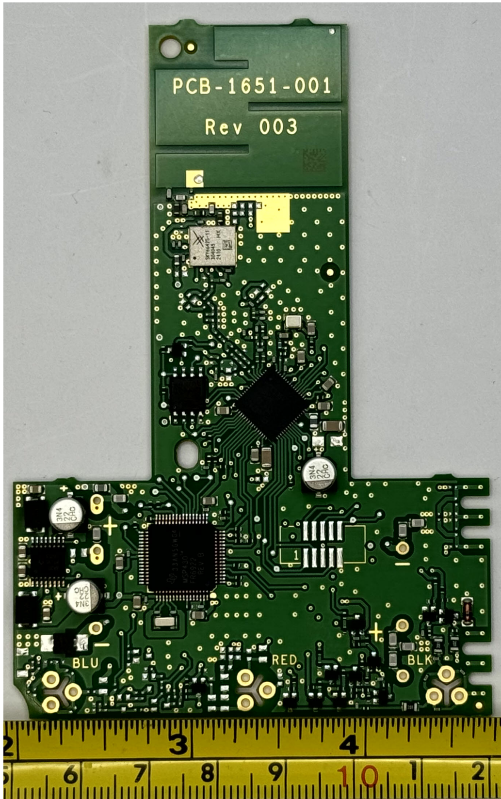
Figure 2.3: Remote Mount - PCB Front, no wires
