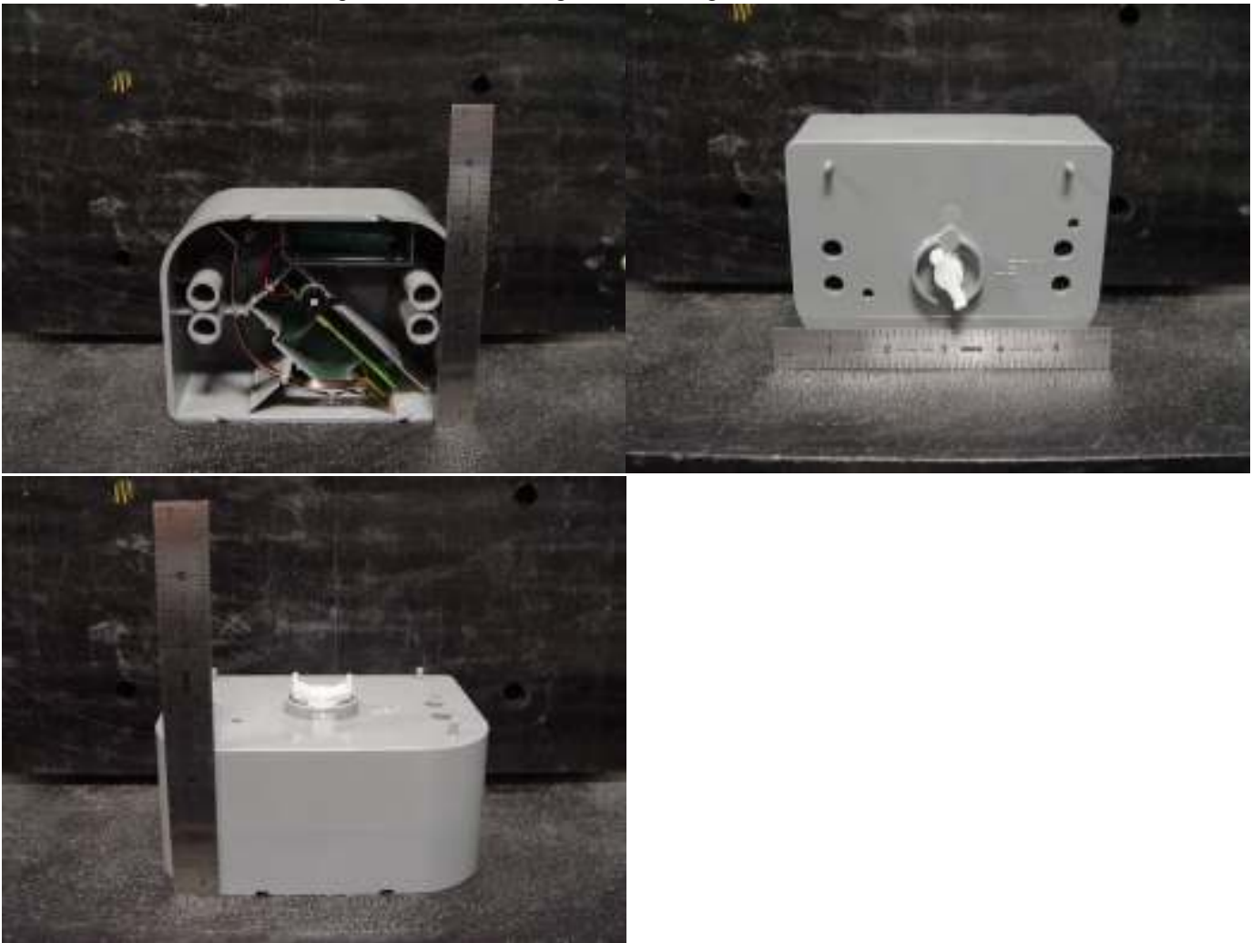
Rockwell Sensus Commercial Endpoint Dimensions Length, Width, Height
