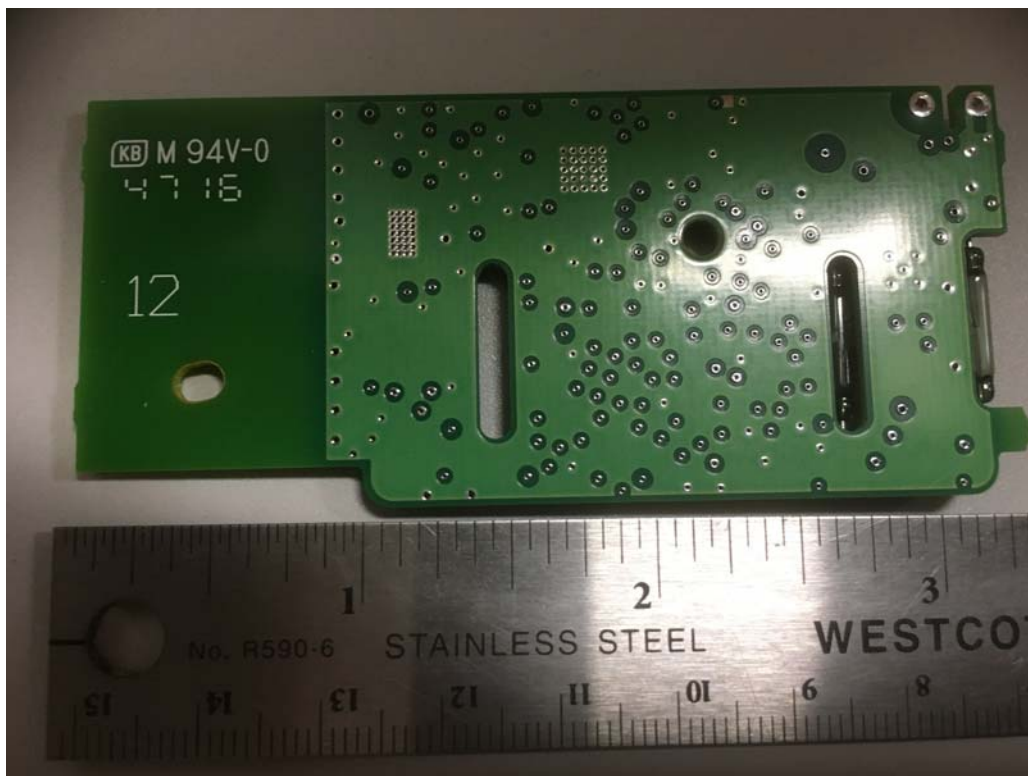
Figure 2 Bottom Side
