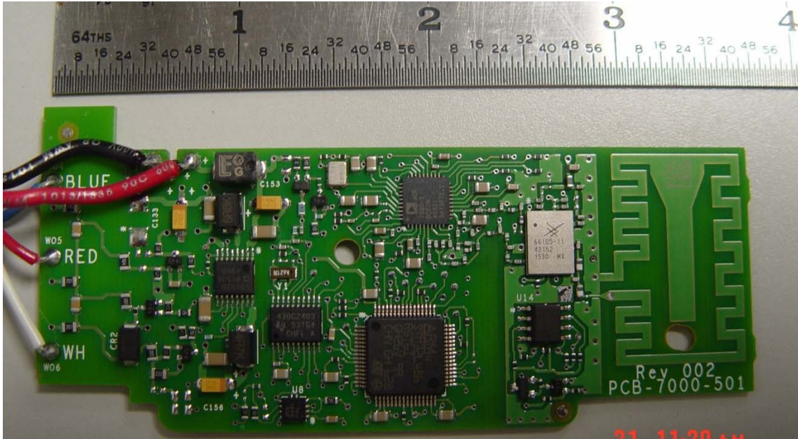
Top Side of PCB-7000-501 used in 500GR
