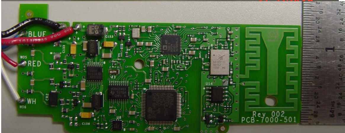
Bottom Side of PCB-7000-501 used in 500GR
