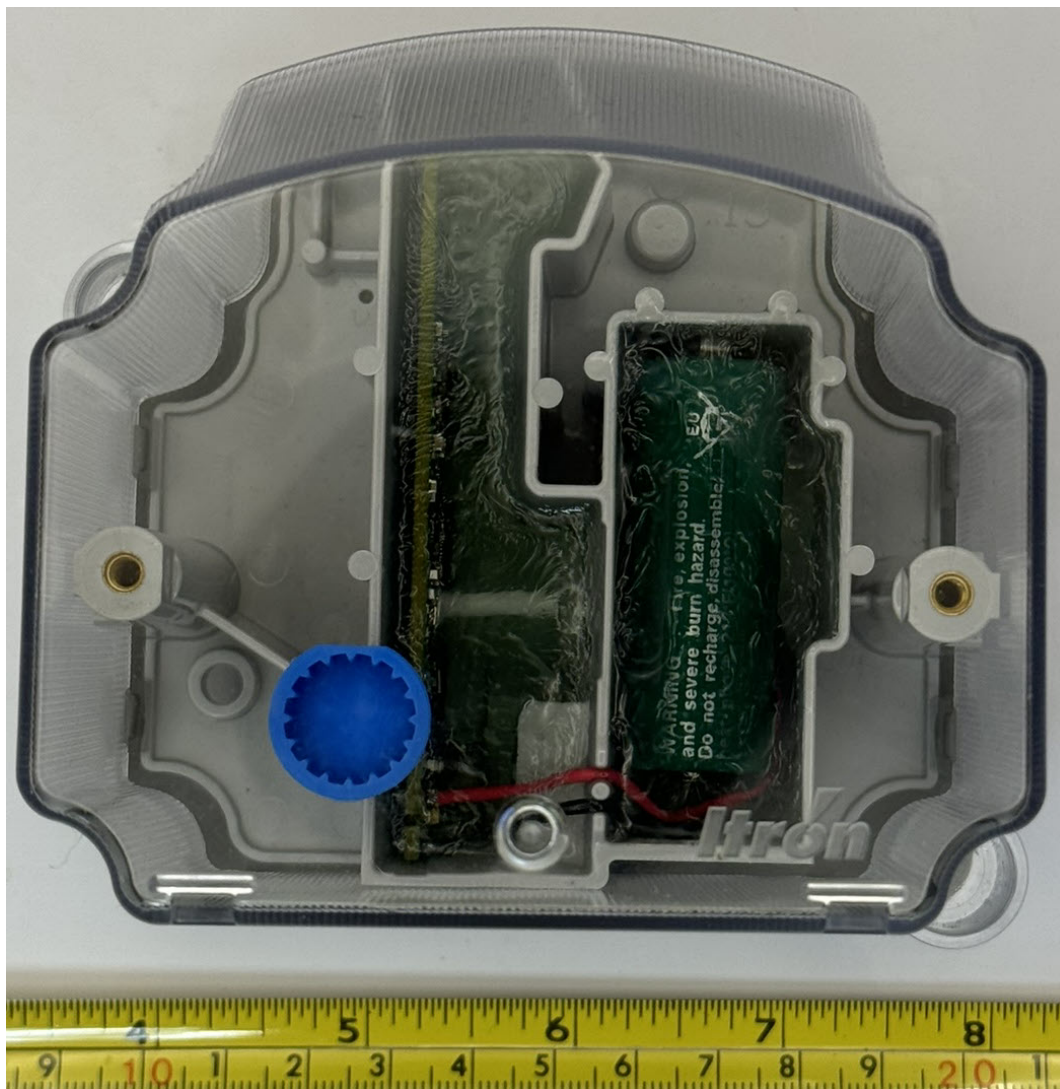
Figure 4.1: ERG-7600-003 External Front
