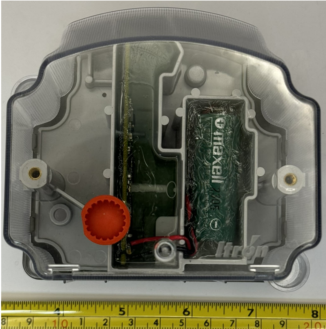
Figure 5.1: ERG-7600-004 External Front
