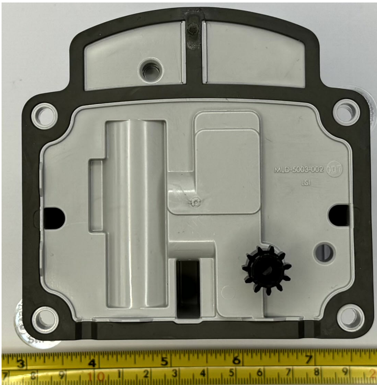
Figure 3.4: ERG-7600-002 External Back
