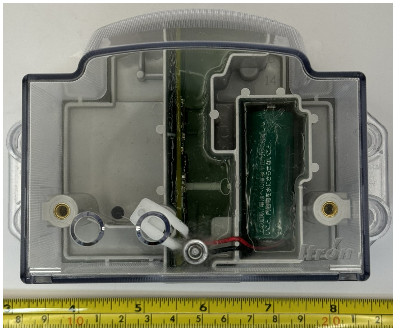
Figure 2.1: ERG-7600-001 External Front
