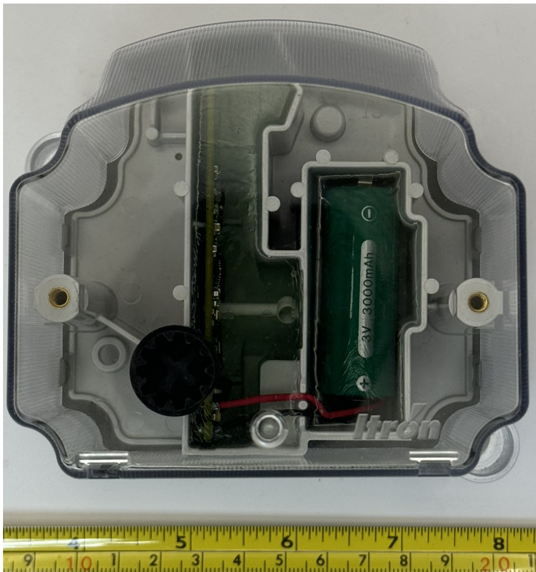
Figure 3.1: ERG-7600-002 External Front
