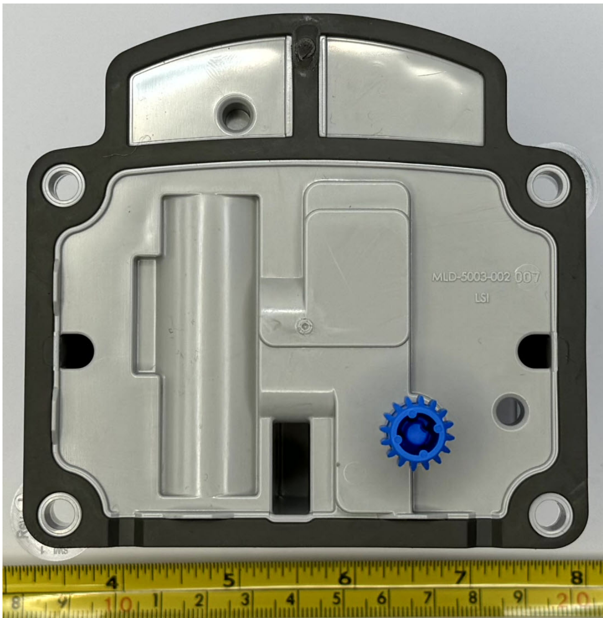
Figure 4.4: ERG-7600-003 External Back
