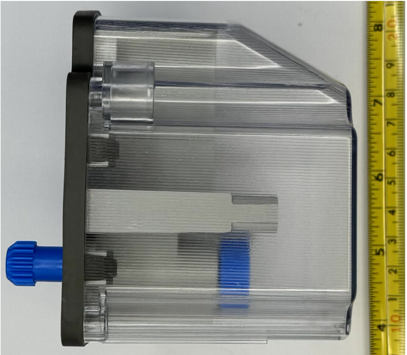
Figure 4.2: ERG-7600-003 External Left
