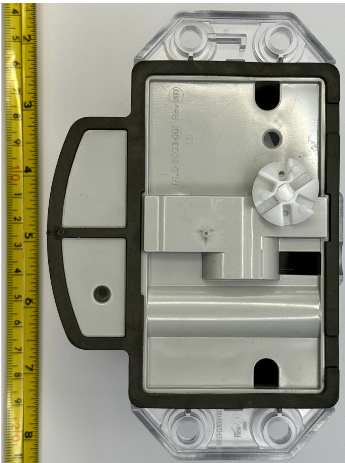
Figure 2.4: ERG-7600-001 External Back
