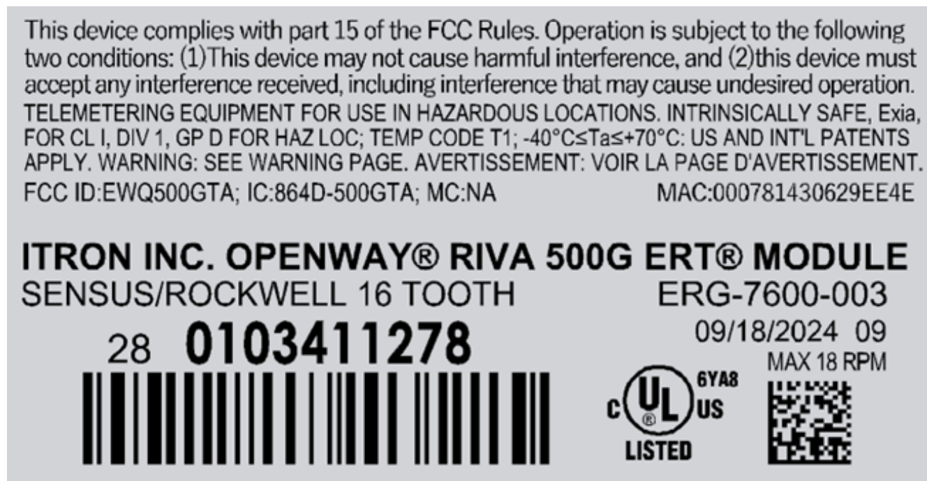
Figure 4.1: ERG-7600-003 Label
