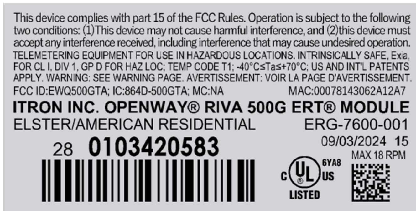
Figure 2.1: ERG-7600-001 Label
