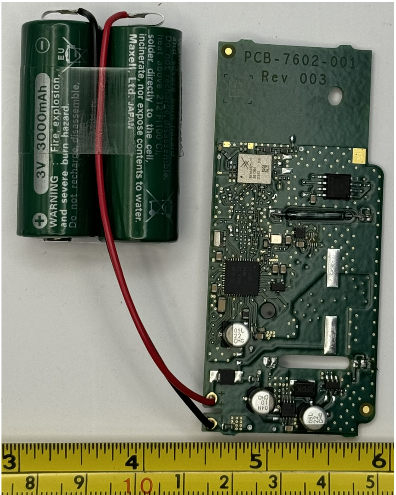
Figure 1.1: PCB Front
