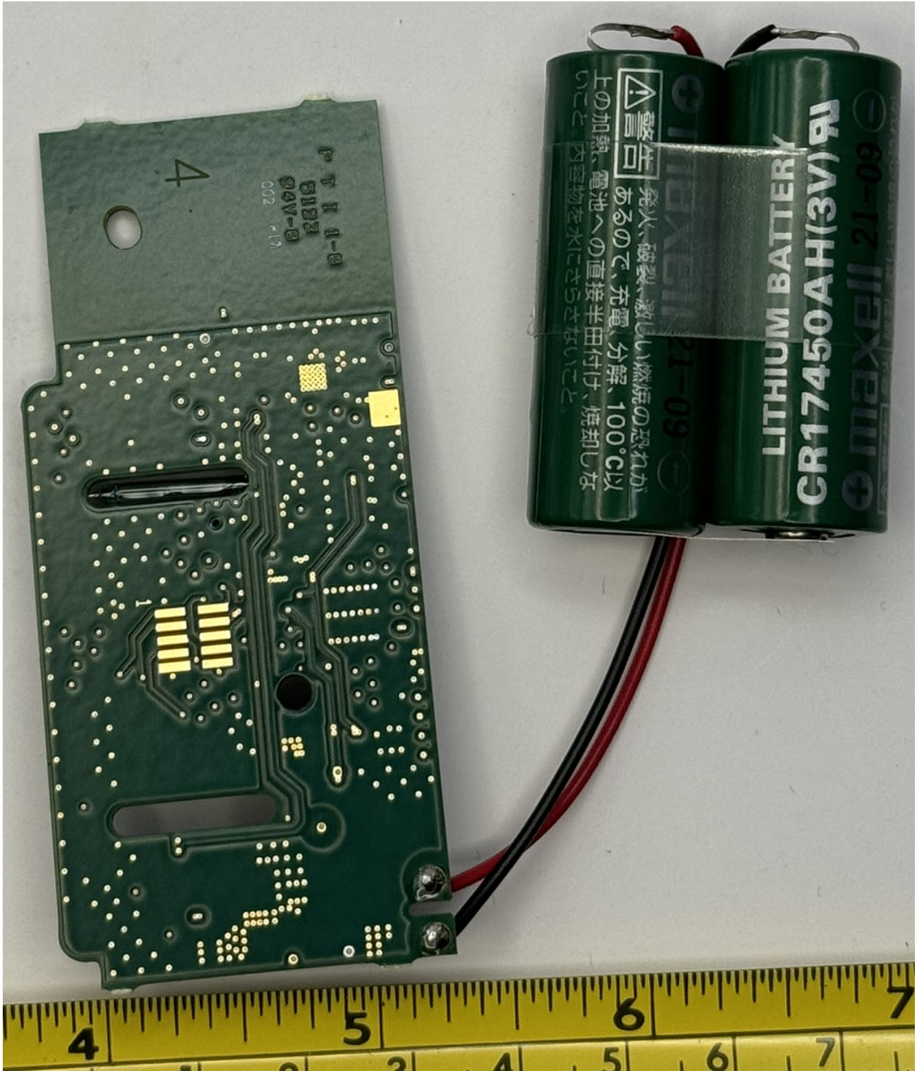
Figure 1.2: PCB Back
