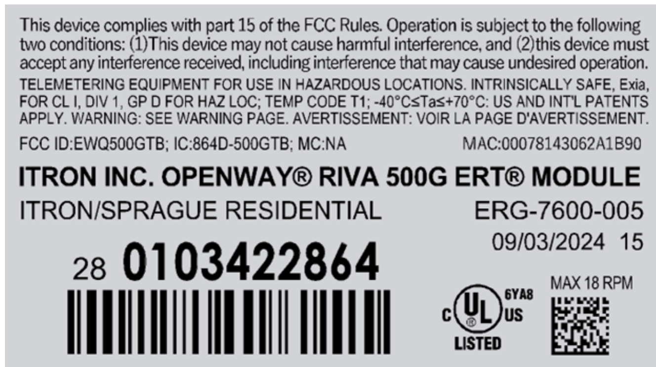
Figure 2.1: ERG-7600-005 Label
