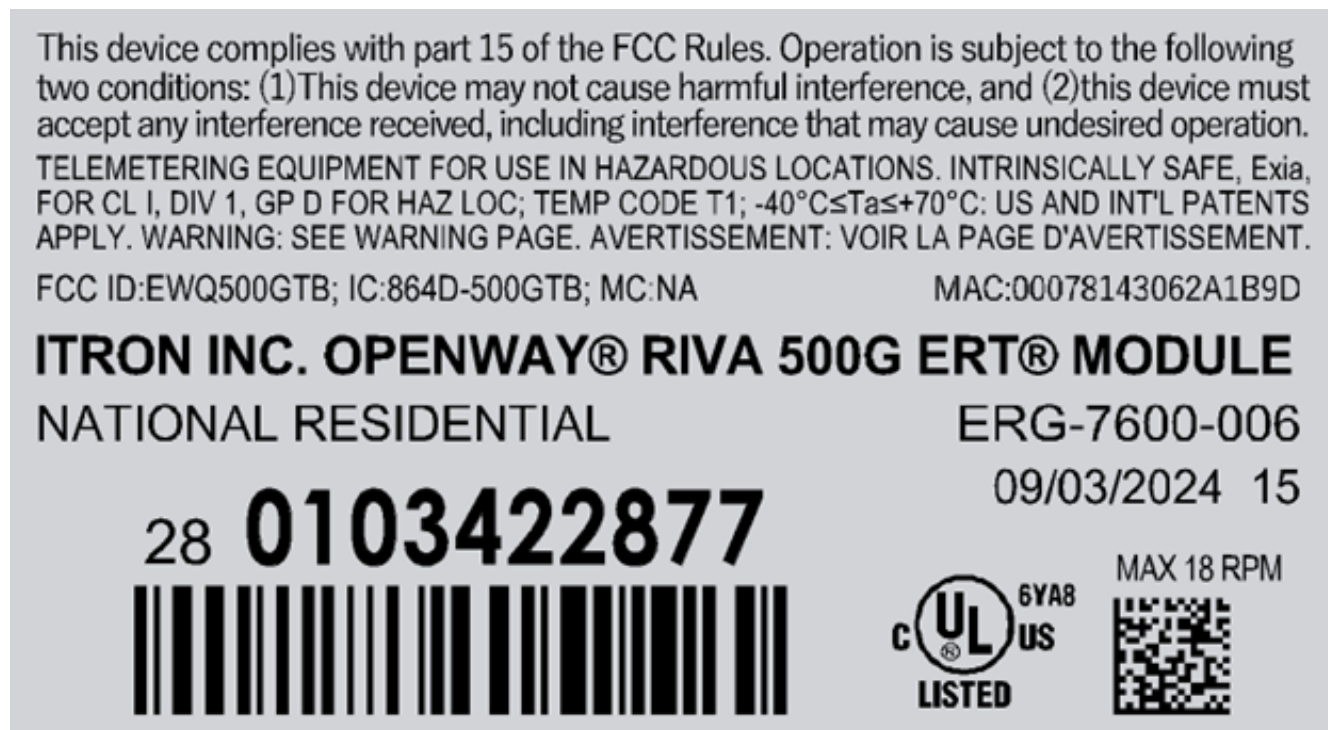
Figure 3.1: ERG-7600-006 Label
