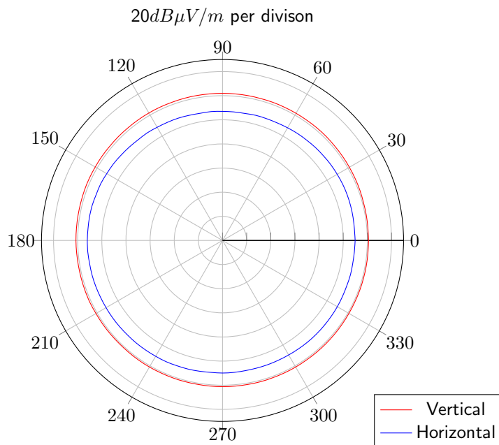
Figure 2: Radiation Pattern
