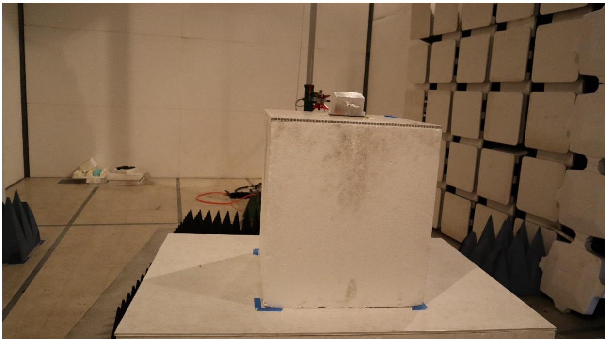
Spurious Emissions ERG-7600-005, 1-18GHz Front
