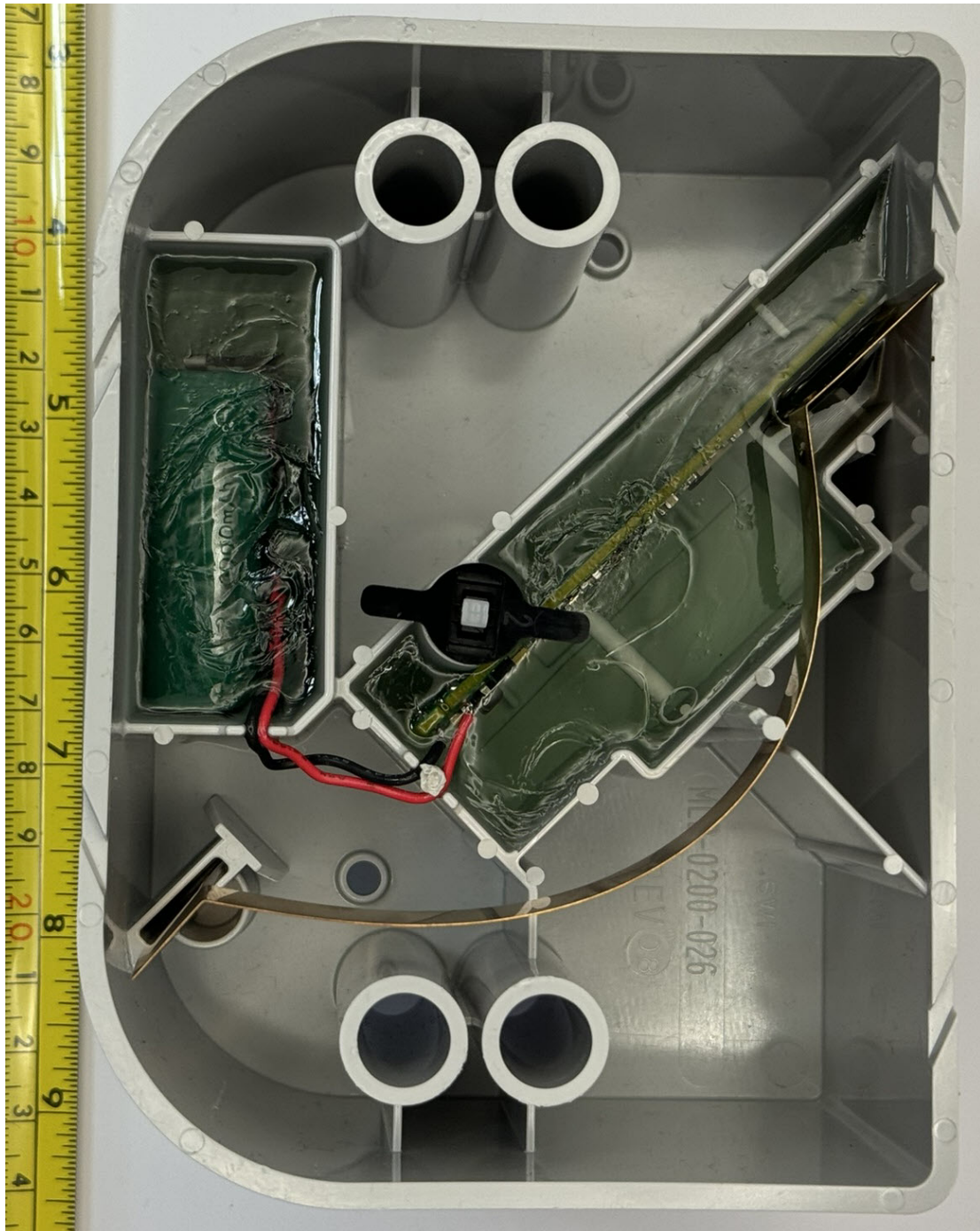
Figure 3.6: ERG-7600-008 External Bottom
