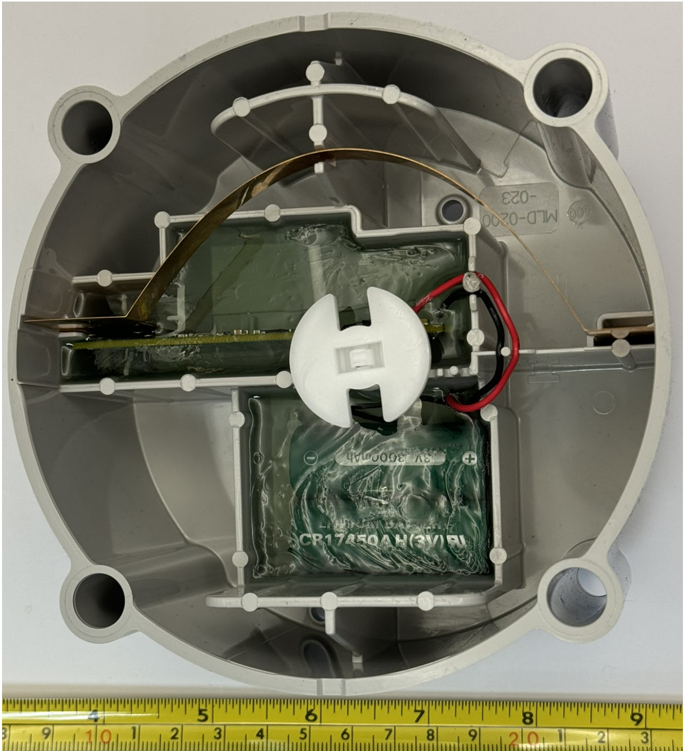
Figure 2.6: ERG-7600-007 External Bottom
