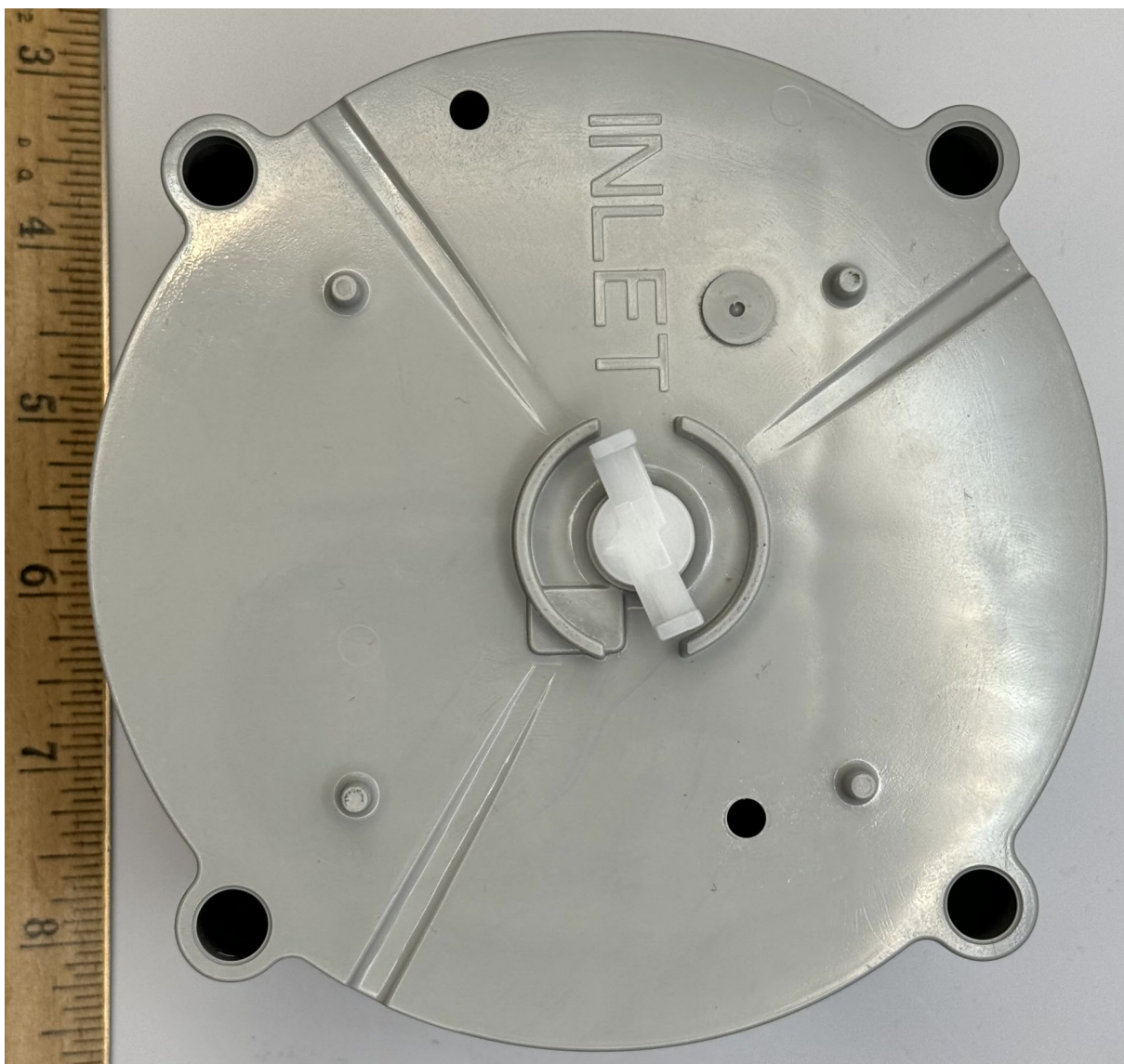
Figure 2.5: ERG-7600-007 External Top
