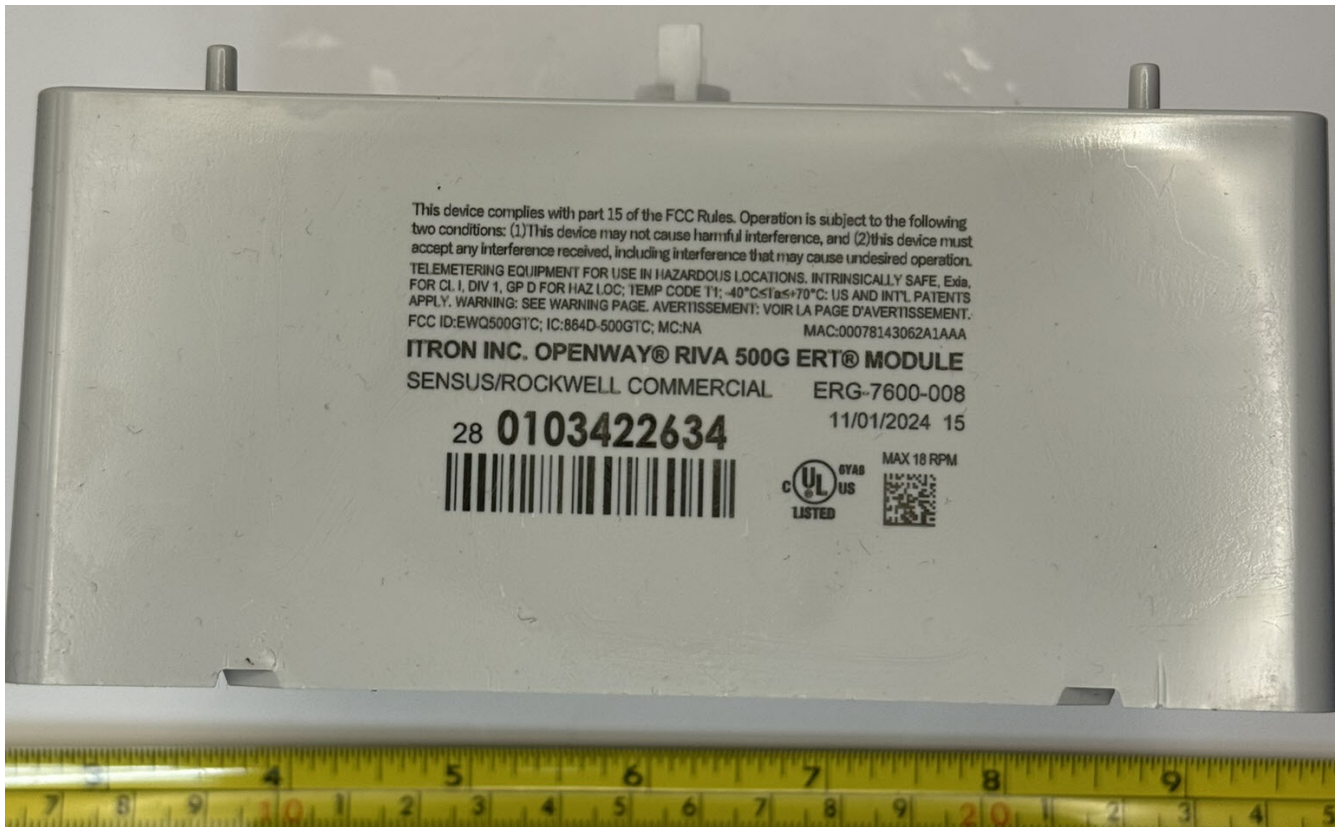
Figure 3.1: ERG-7600-008 External Front
