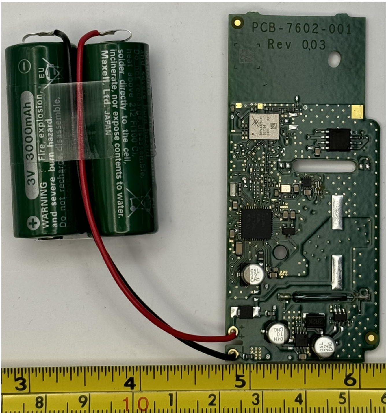
Figure 1.1: PCB Front
