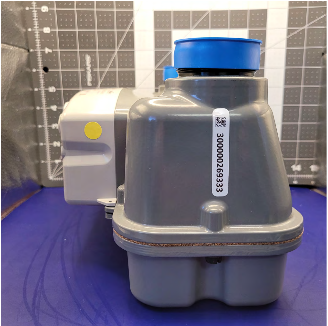
Figure 4.15: Meter 425 8.25" - Right
