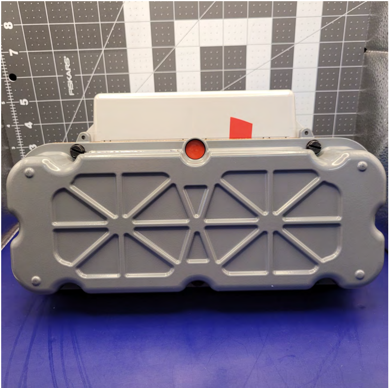
Figure 4.18: Meter 425 8.25" - Bottom
