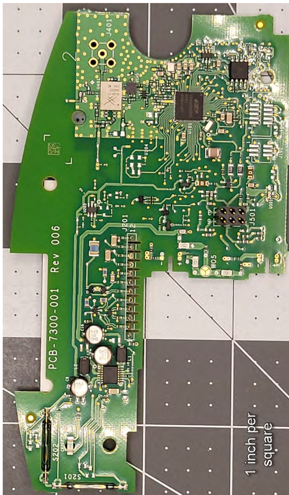
Figure 2.1: Electronic Index PCB Front
