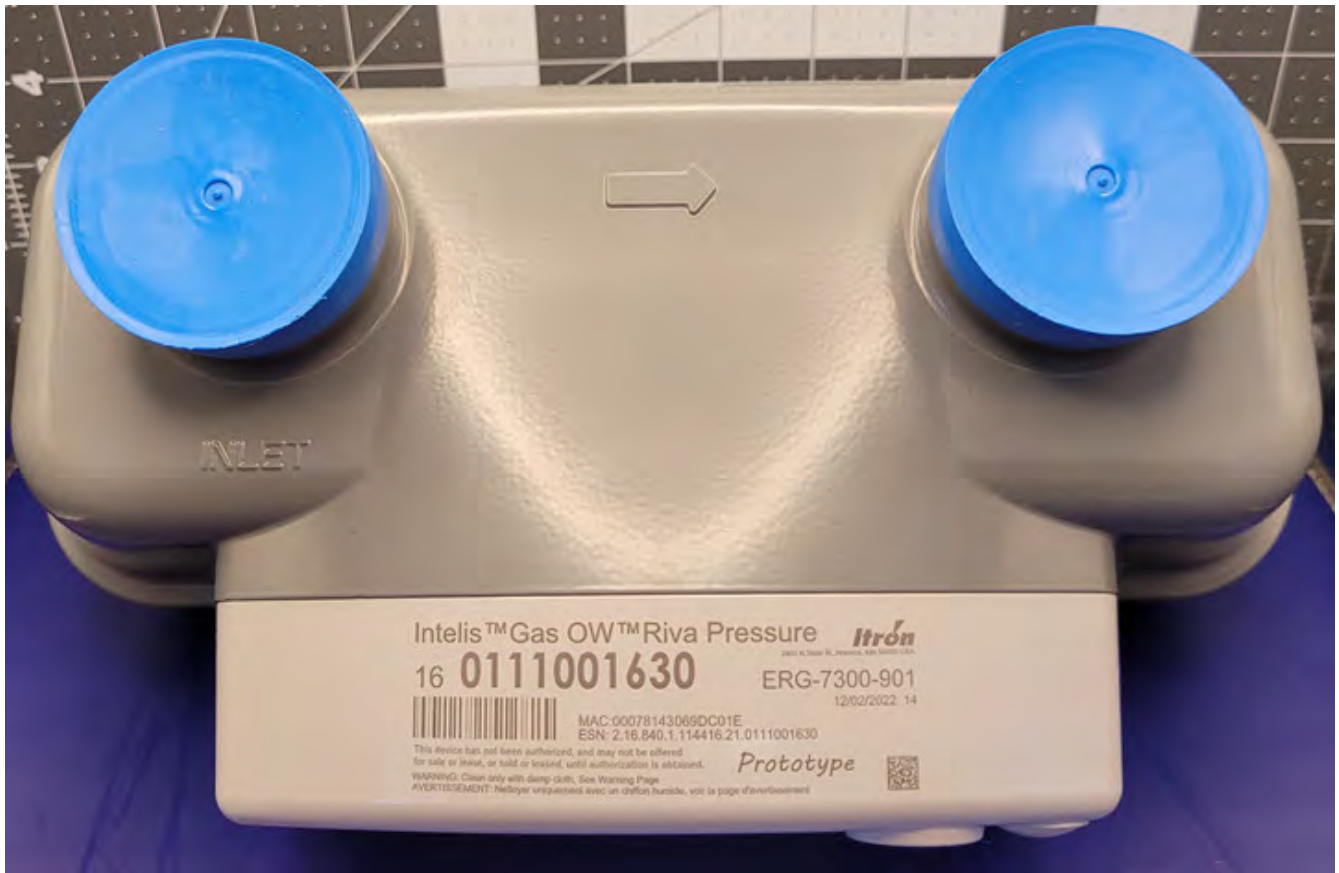
Figure 4.11: Meter 425 6" - Top
