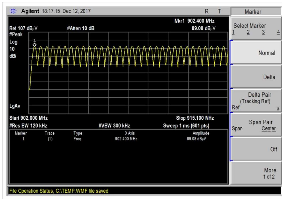
GFSK_150kbps_LowMid_32CH
