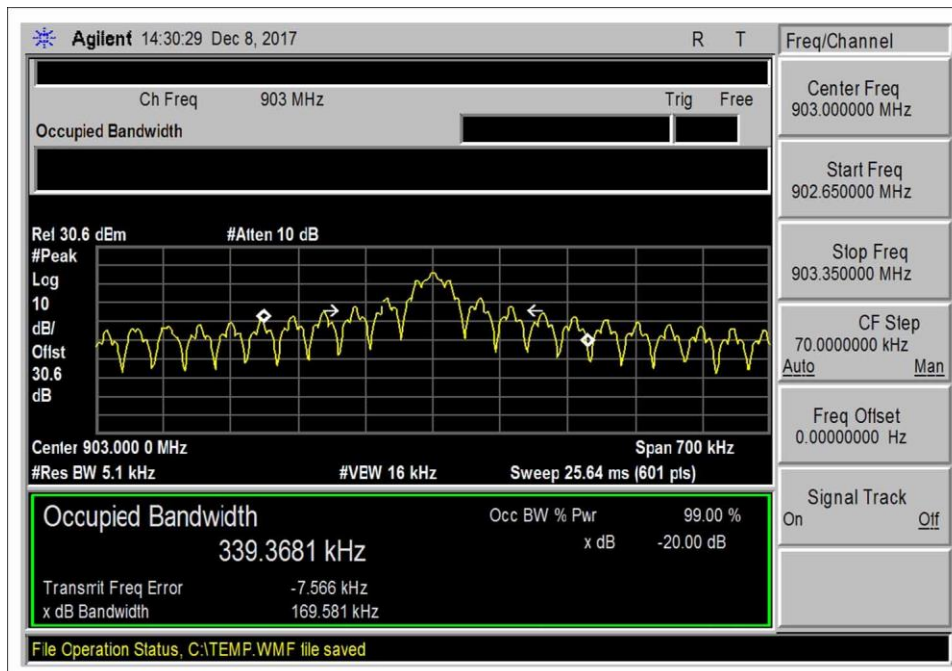
20db_BW_OOK_pl3_lowCH
