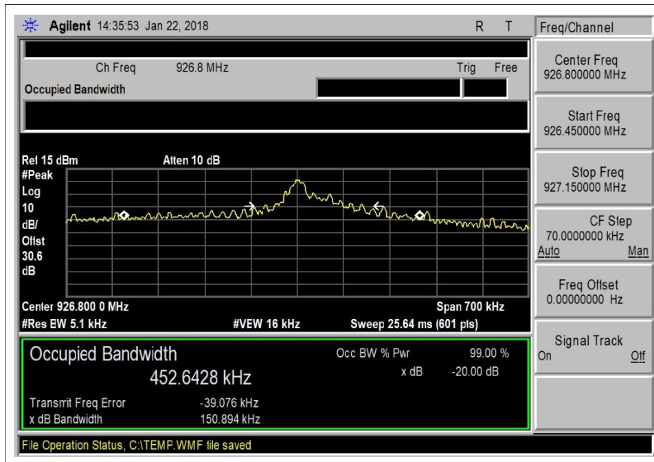
20db_BW_OOK_pl1_highCH
