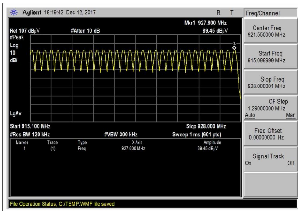
GFSK_150kbps_MidHigh_32CH
