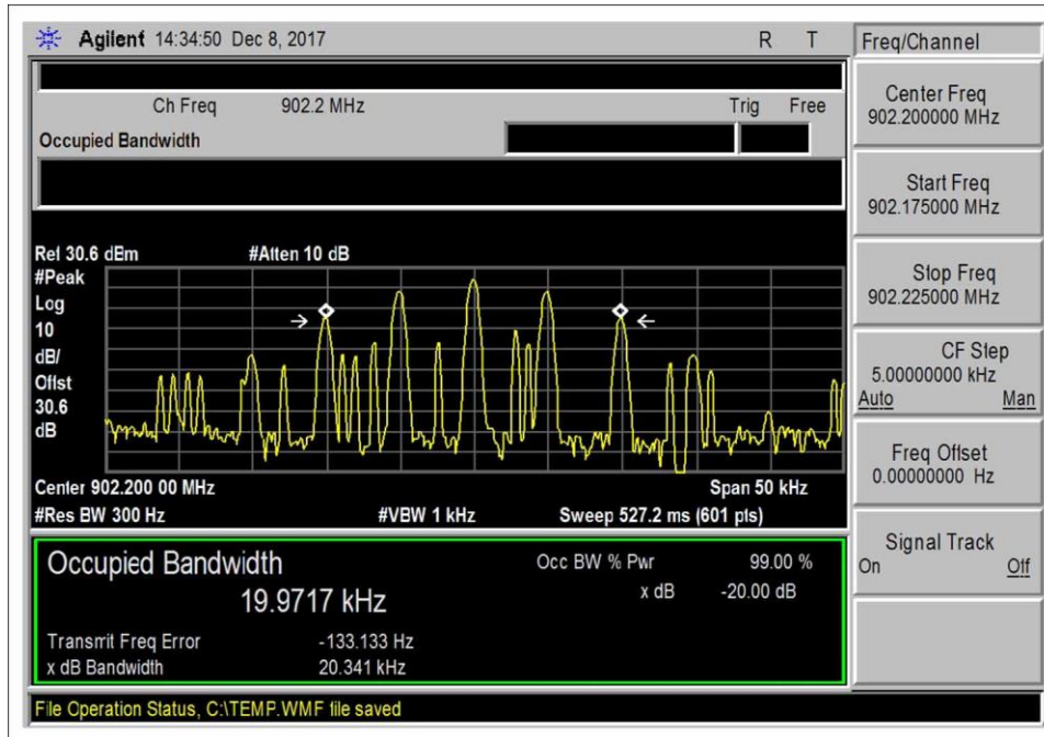
20db_BW_GFSK_10kbps_pl3_lowCH
