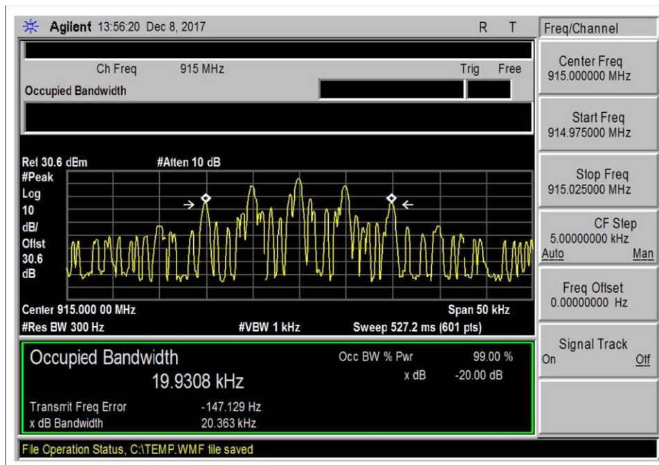
20db_BW_GFSK_10kbps_pl3_midCH
