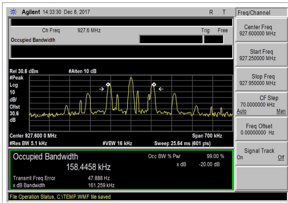
20db_BW_GFSK_150kbps_pl3_highCH
