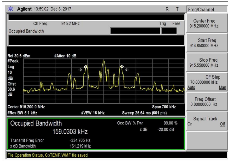
20db_BW_GFSK_150kbps_pl3_midCH
