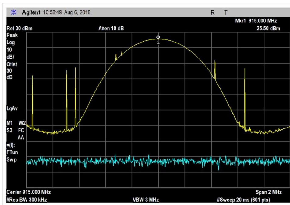
GFSK 10kbps, Power 3, Vertical 915MHz
