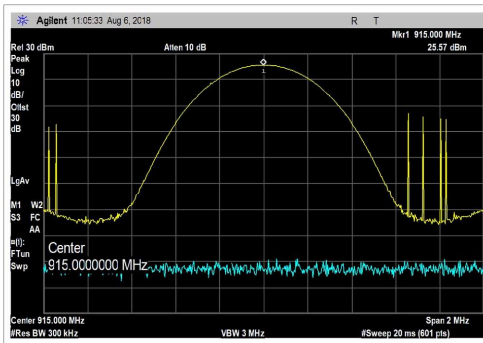
GFSK 10kbps, Power 3, Horizontal 915MHz
