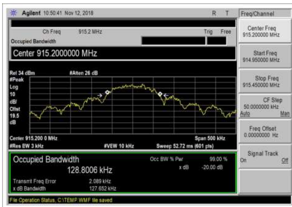
100kbps, Middle Channel, Vertical Pipe
