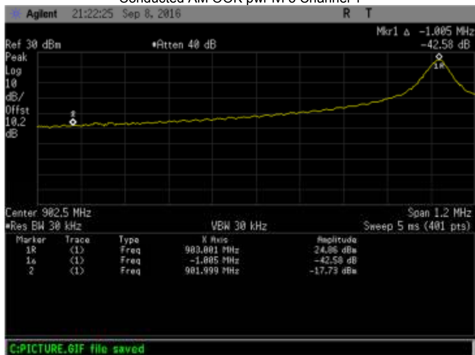
Conducted AM OOK pwr lvl 3 Channel 1
