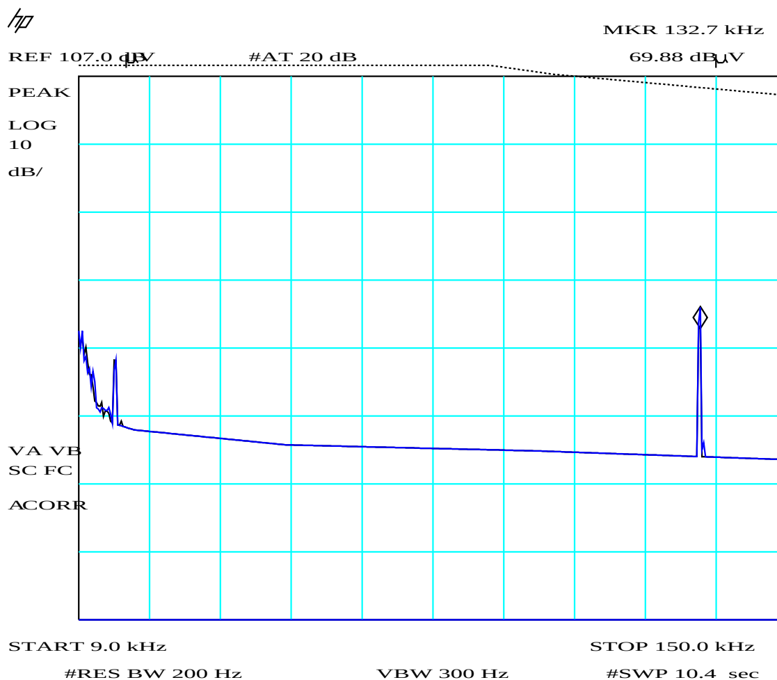
PLOT 11 Radiated Emissions - SP500 - 9kHz to 150kHz (FCC Limit)
