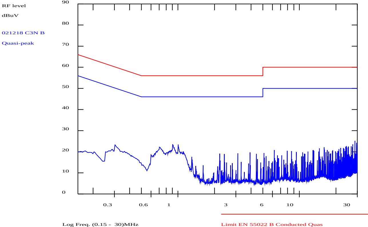
PLOT 3 Conducted Emissions - SP500 115V Neutral
