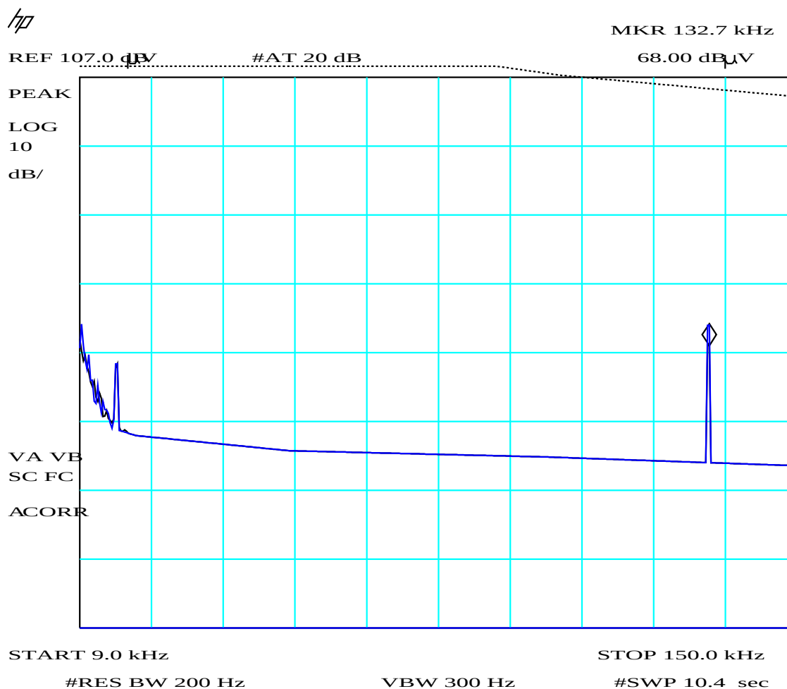
PLOT 15 Radiated Emissions - PM500 - 9kHz to 150kHz (FCC Limit)
