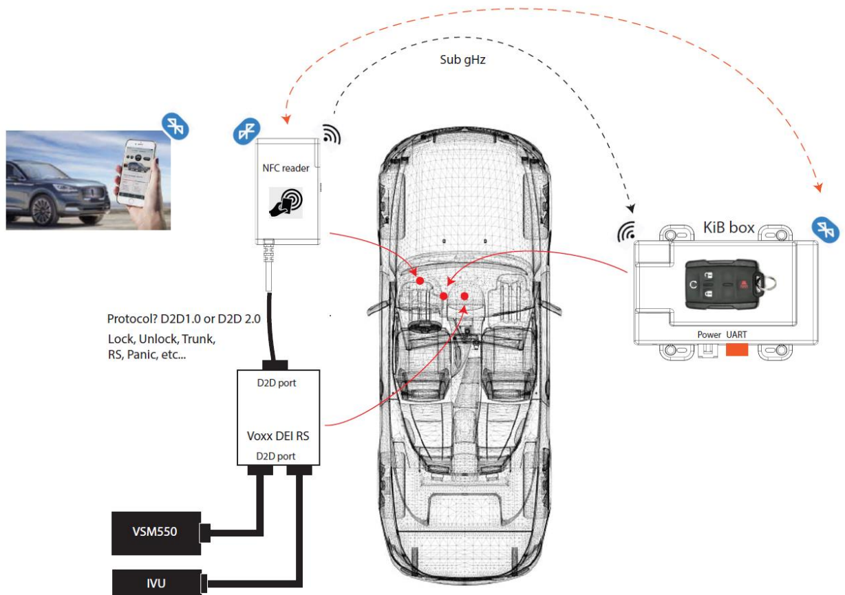
Figure 1 EKey System Diagram
