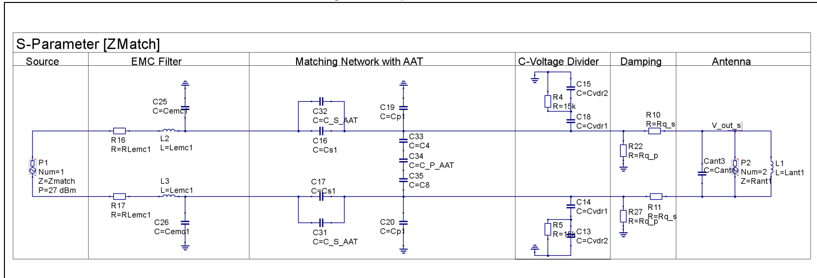
Figure 22. S-parameter model
