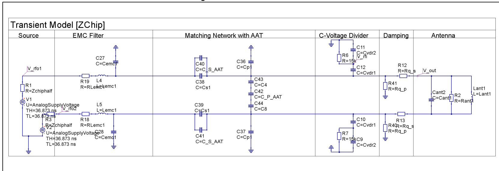
Figure 23. Transient simulation
