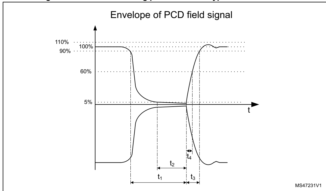
Figure 9. Definition of timing parameters for Type-A with 106 kbit/s
