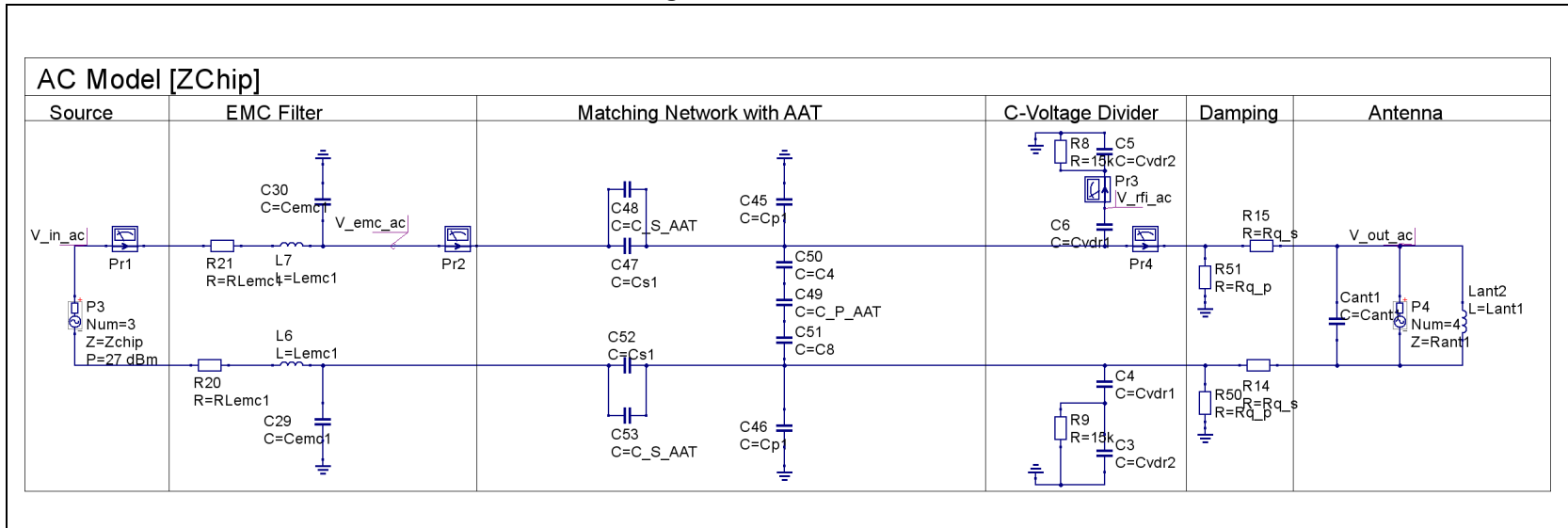
Figure 24. AC simulation
