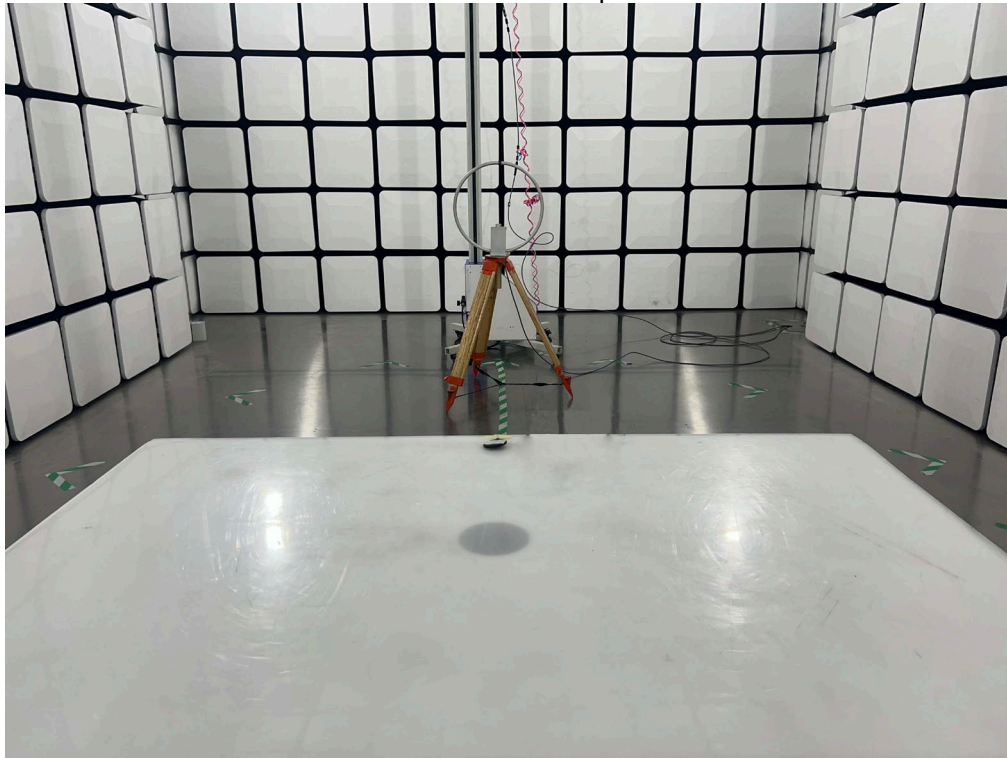
RFID Test set-up
