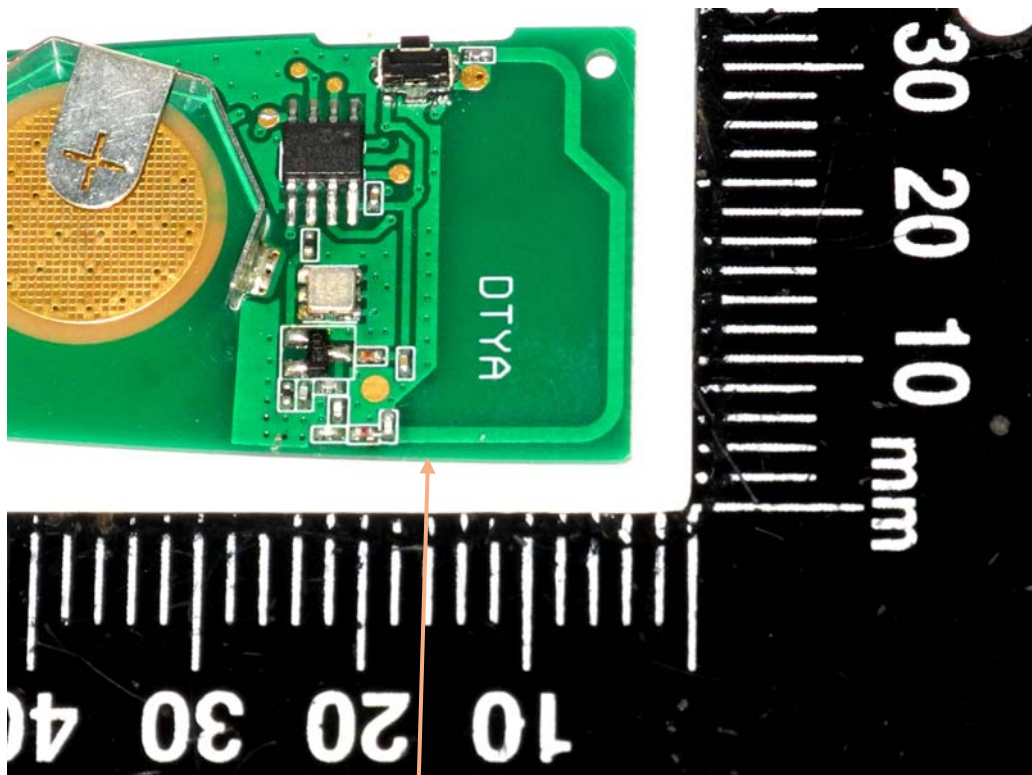
Antenna location
