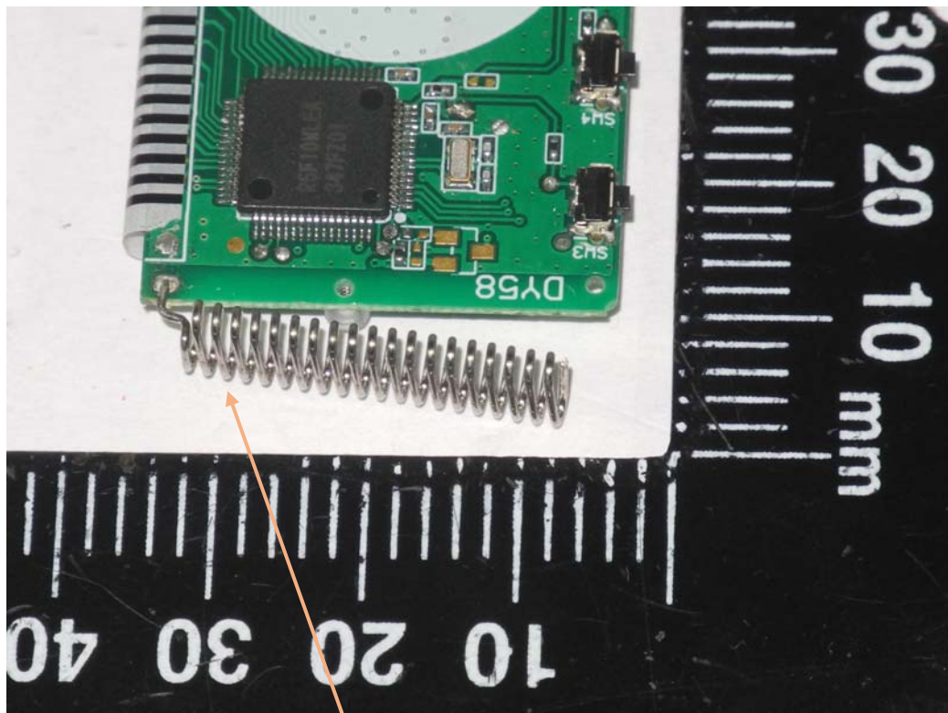
Antenna location
