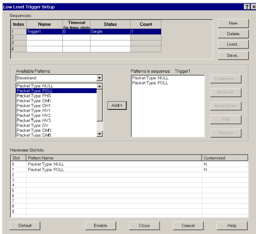
Figure 1-6: Low Level Trigger Setup dialog box
