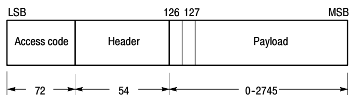
Figure 2-7: Standard packet format
