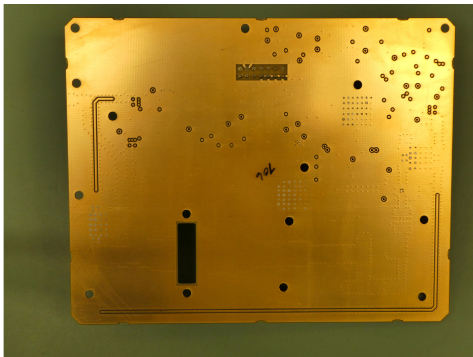
Power Amplifier PCBA 3-26070-3 Rear view
