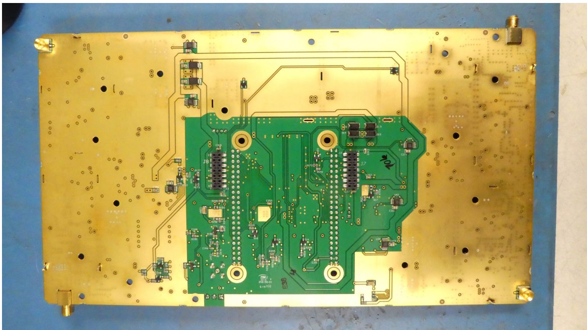
Control and LNA PCBA 3-26063-1 Rear view
