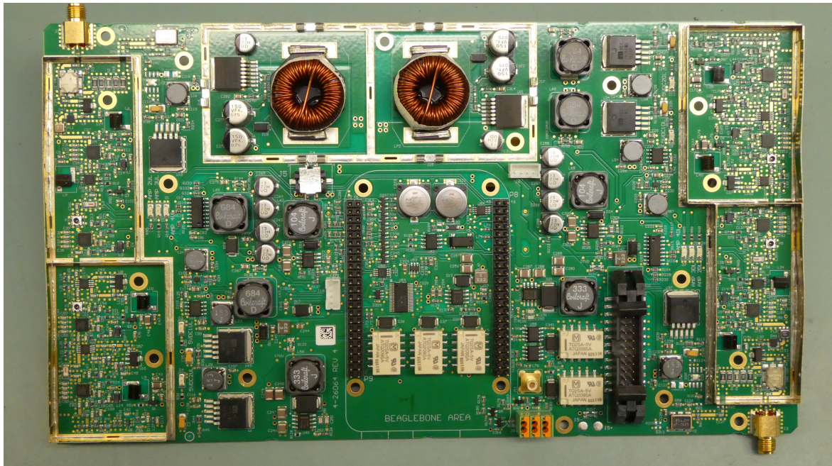
Control and LNA PCBA 3-26063-1 Front view
