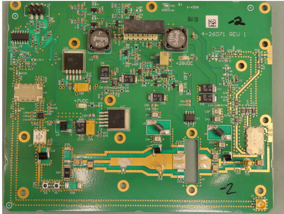
Power Amplifier PCBA 3-26070-2 Front view
