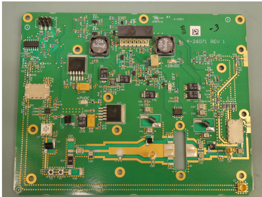
Power Amplifier PCBA 3-26070-3 Front view
