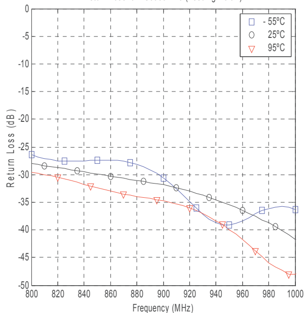
Return Loss for XC0900A-20 (Feeding Port 4)
