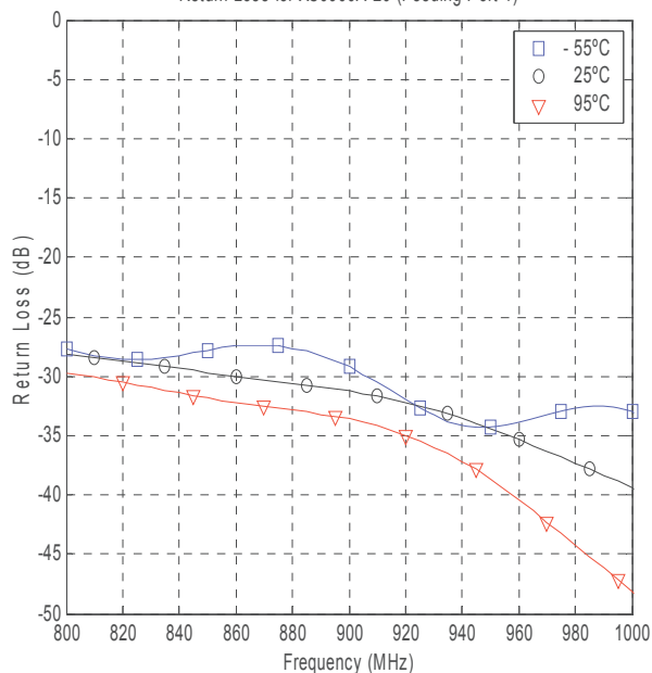
Return Loss for XC0900A-20 (Feeding Port 1)
