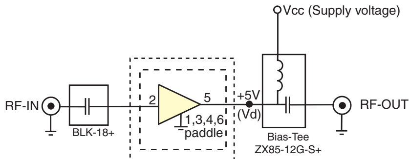
Fig 1. Block Diagram of Test Circuit used for characterization. (DUT soldered on Mini-Circuits Characterization test board TB-641-1+) Gain, Return loss, Output power at 1dB compression (P1 dB), output IP3 (OIP3) and noise figure measured using Agilent's N5242A PNA-X microwave network analyzer.
