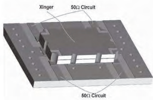
Figure 3: Component Placement
