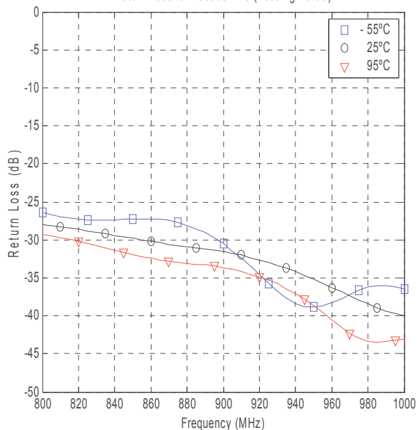
Return Loss for XC0900A-20 (Feeding Port 3)
