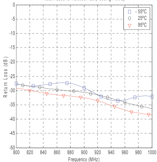
Return Loss for XC0900A-20 (Feeding Port 2)
