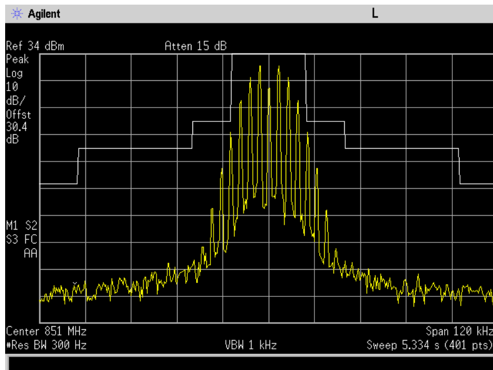
Downlink 851_Mask B
