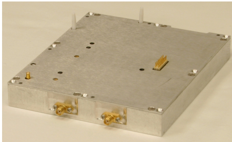
Downlink Power Amplifier Assembly 3-26069-1 Side view.
