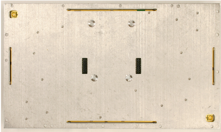
Control and LNA Assembly 3-26062-2, or 3-26062-3, or 3-26062-4 Bottom view.
