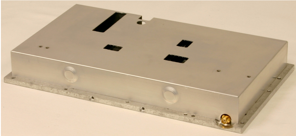
Control and LNA Assembly 3-26062-2, or 3-26062-3, or 3-26062-4 Rear-side view.
