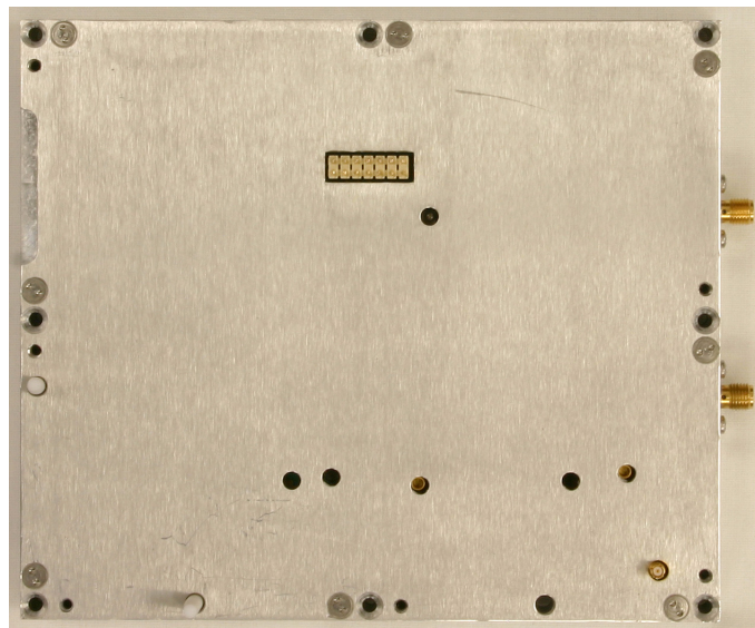
Downlink Power Amplifier Assembly 3-26069-1 Top view.
